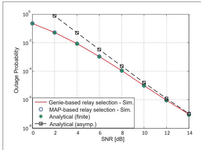
Figure 4.11 End-to-end outage performances of various N 'th BRS schemes with M = 5 relays over Rayleigh faded TSMG channels. A system involving an uncoded transmission and a BPSK modulation is considered
