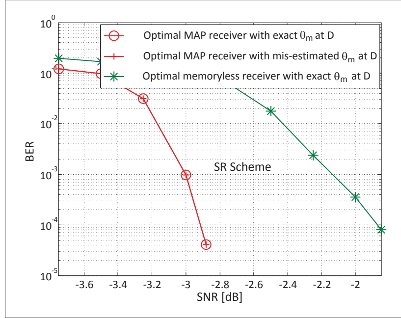
Figure 3.9 BER performances of coded simple relaying (SR) scheme assuming different realizations of \theta_m at the destination. A BPSK modulation is adopted and each channel is characterized by p_B = 0.1 , \gamma = 100 , R = 100
