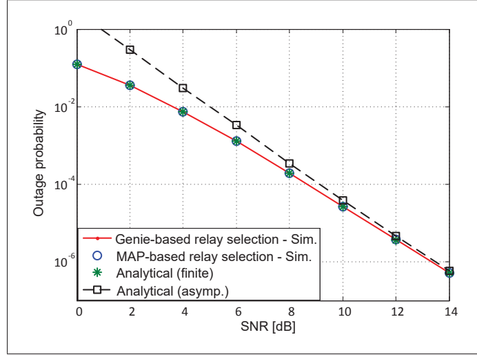
Figure 4.10 Outage performances at the N 'th best relay of various relay selection schemes with M = 5 relays over Rayleigh faded TSMG channels. A system involving an uncoded transmission and a BPSK modulation is considered
