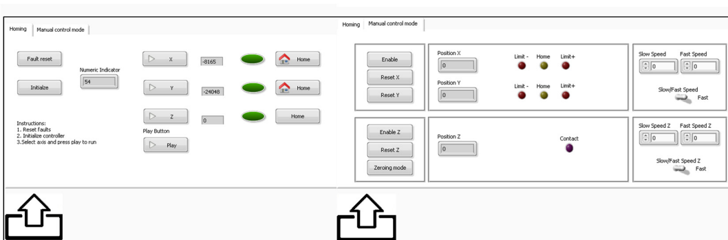
Figure 4.5 : Machine calibration virtual instrument (2 instrument page tab)
