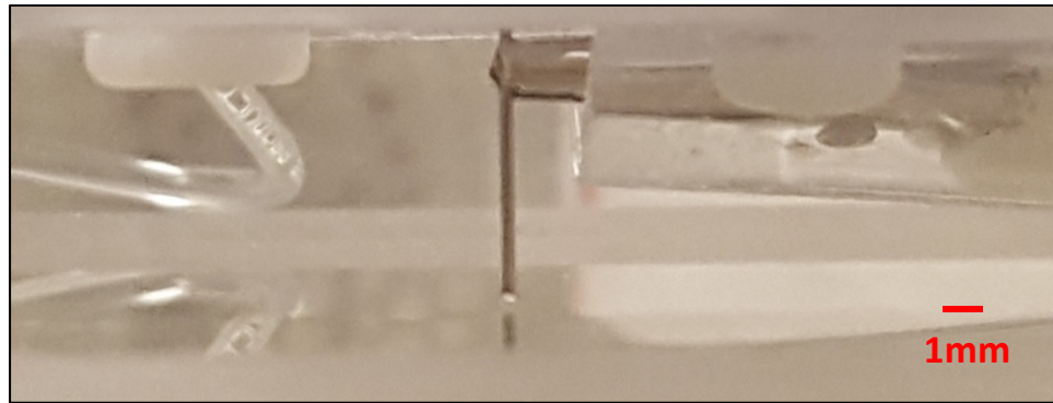
Figure 4.6 : Fluid preload, hemisphere droplet at end of dispensing needle
