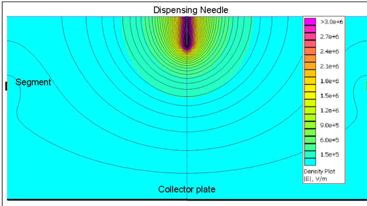
Figure 1.6: Intrusion of a grounded element in the electric field
