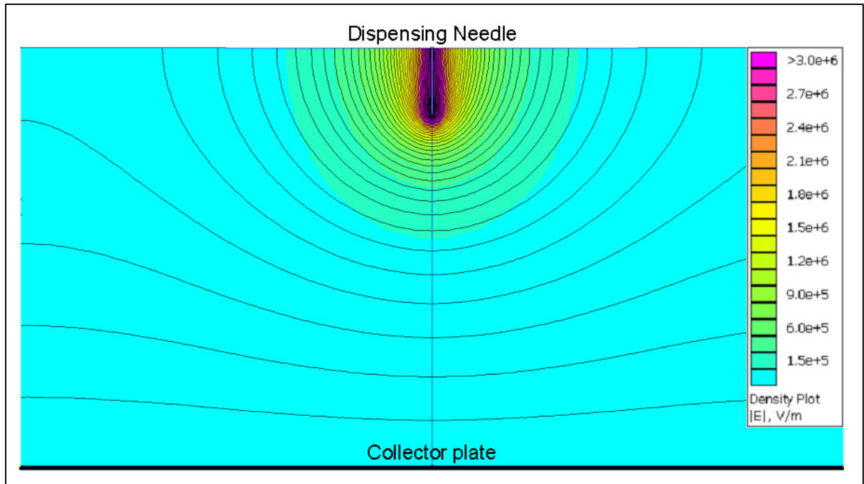
Figure 1.2: Voltage distribution of a fixed collector setup
