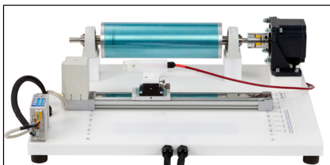
Figure 1.8: Typical drum collector setup Spraybase®
