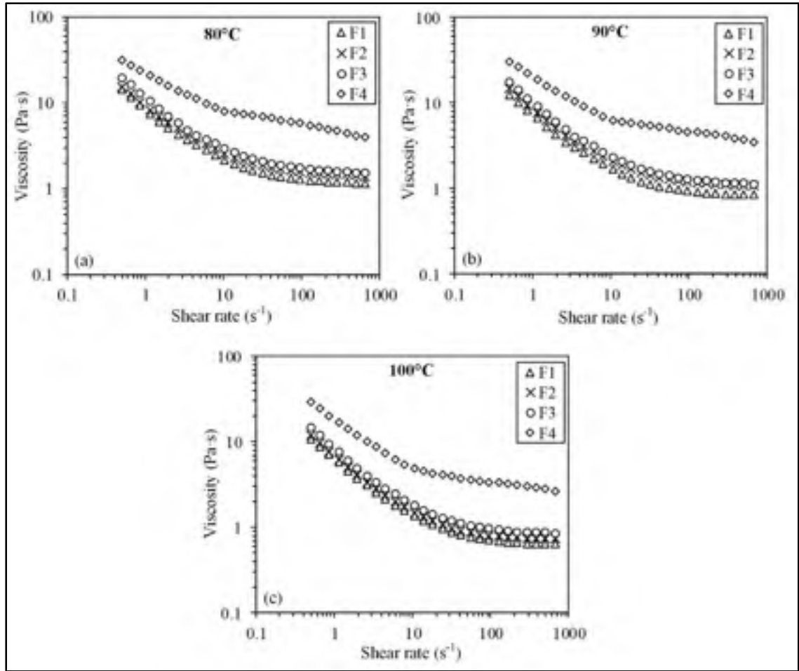
Figure 4.3 Viscosity profiles of feedstocks F1, F2, F3, and F4 at (a) 80 °C, (b) 90 °C, and (c) 100 °C
