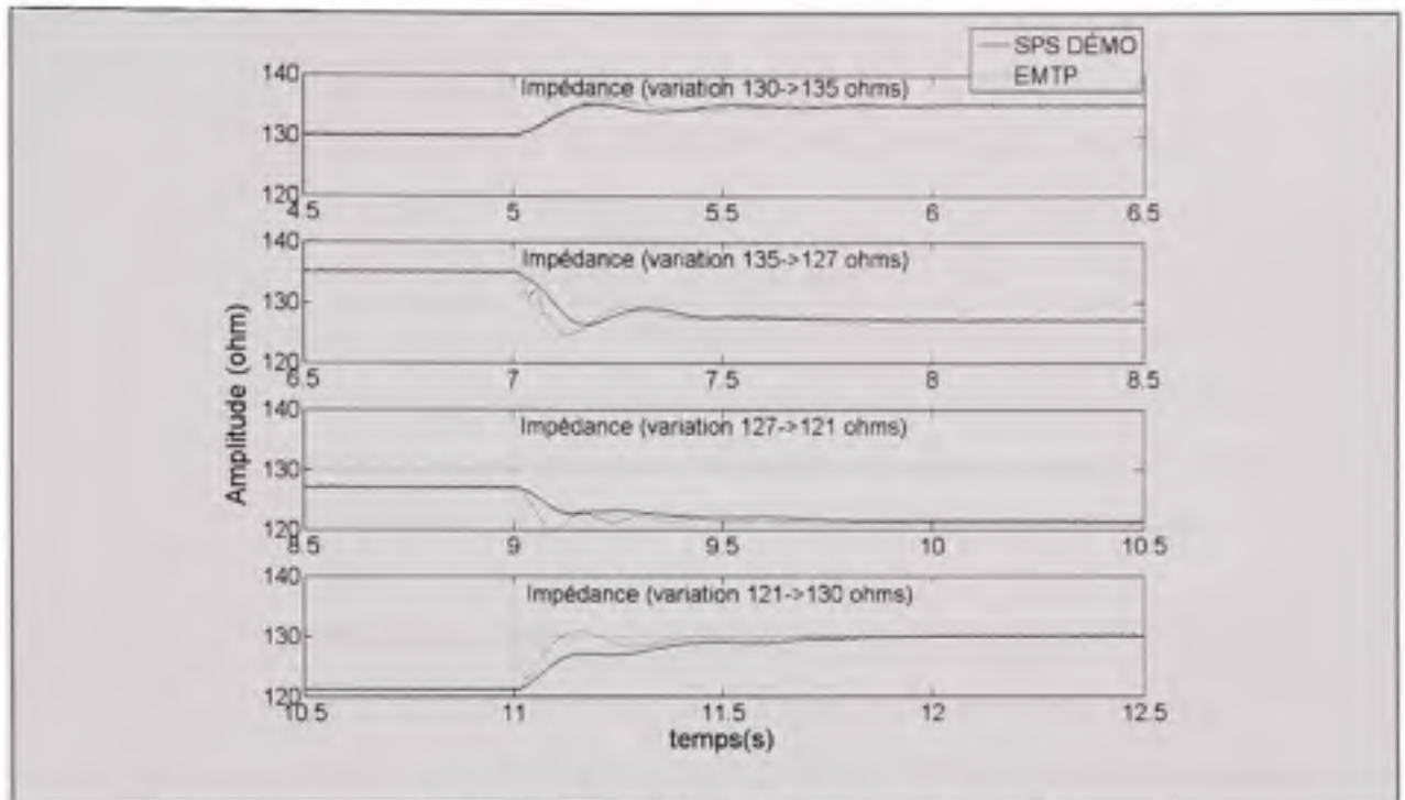
Figure 4-33 Comparaison impédance.
