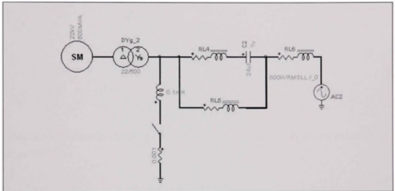
FigureAppendice I.1 Second banc d'essai
