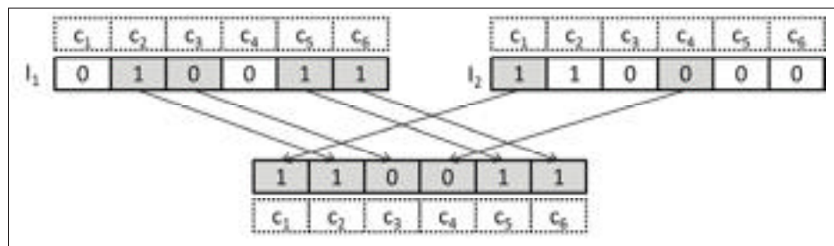
Figure 4.6 Evolution-based crossover.
