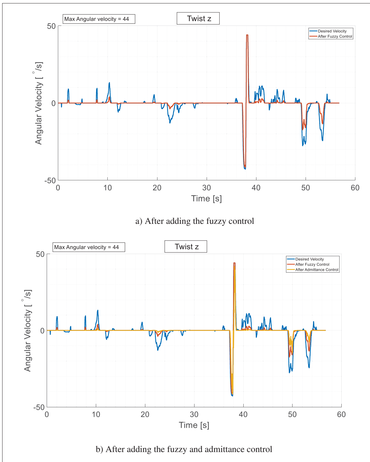
Figure 5.16 Robot's performance at a desired angular velocity of maximum 44^{\circ}/s while twisting in z-direction after adding the proposed controllers is series
