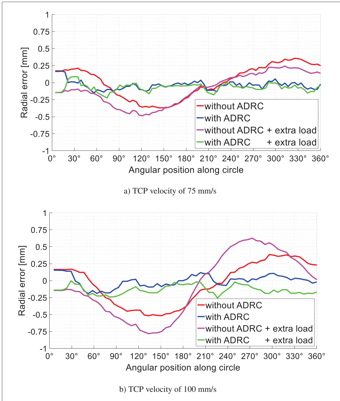
Figure 4.5 Robot's radial error measured with the ballbar at different TCP velocities, with and without ADRC controller, with robot's rated payload (0.5 kg) and with robot's full payload (1 kg), at robot's high speeds
