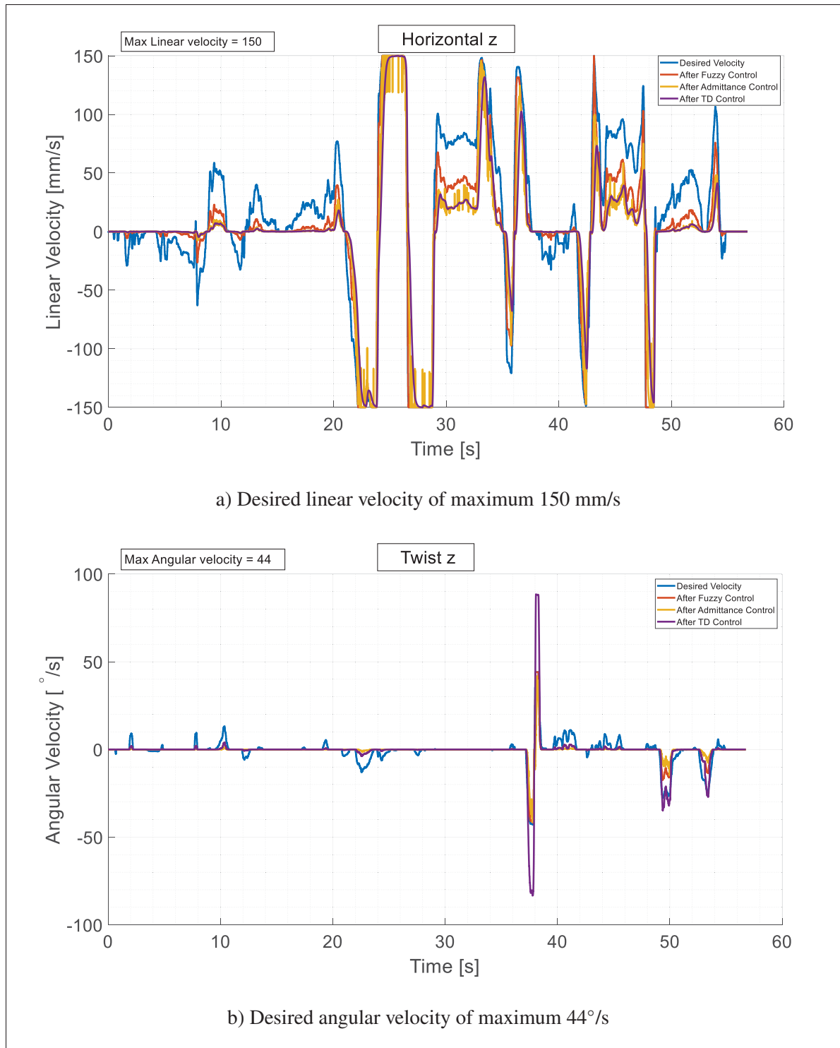
Figure 5.17 Robot's performance at desired maximum linear and angular velocities while moving in horizontal z-direction, and twisting in z-direction, respectively, both after adding the fuzzy, admittance, and TD controllers in series
