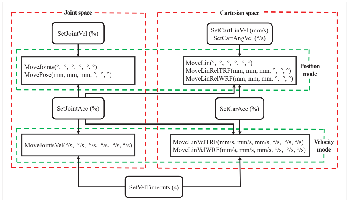
Figure 3.3 Settings that influence the robot motion in position and velocity modes Taken from Mecedemic (2020)
