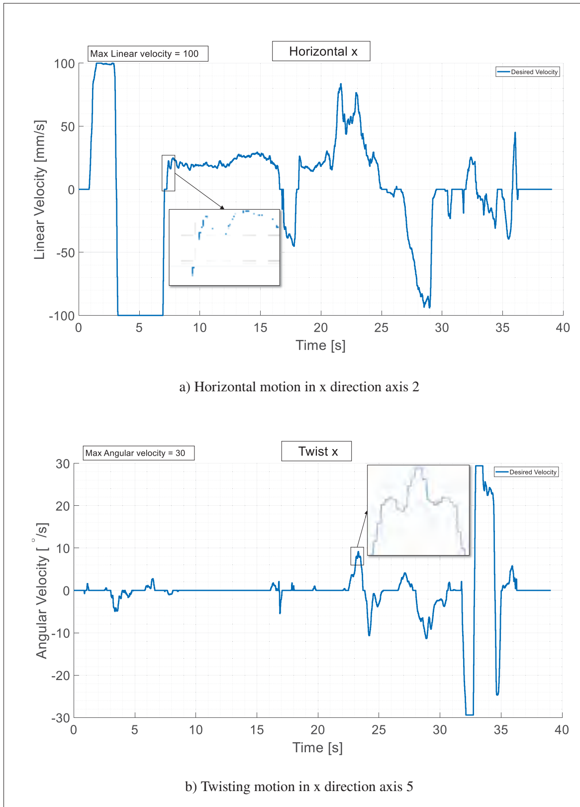
Figure 3.25 Robot's desired motion and twisting in x directions at maximum linear and angular speeds of 100 mm/s and 30 °/s, respectively
