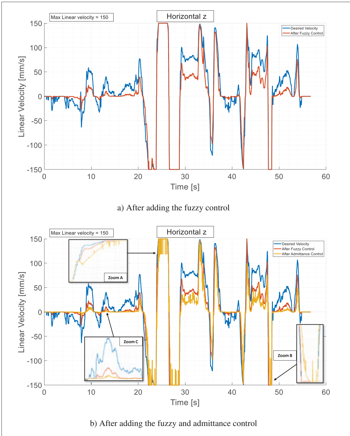
Figure 5.15 Robot’s performance at a desired linear velocity of maximum 150 mm/s while moving in horizontal z-direction after adding the proposed controllers is series
