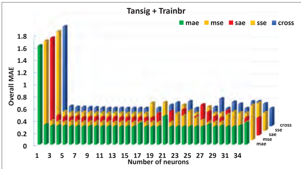
Figure-A I-6 Influence of number of neurons using RMSProp optimizing option with Tansig activation function and trainbr training algorithms with different performance functions
