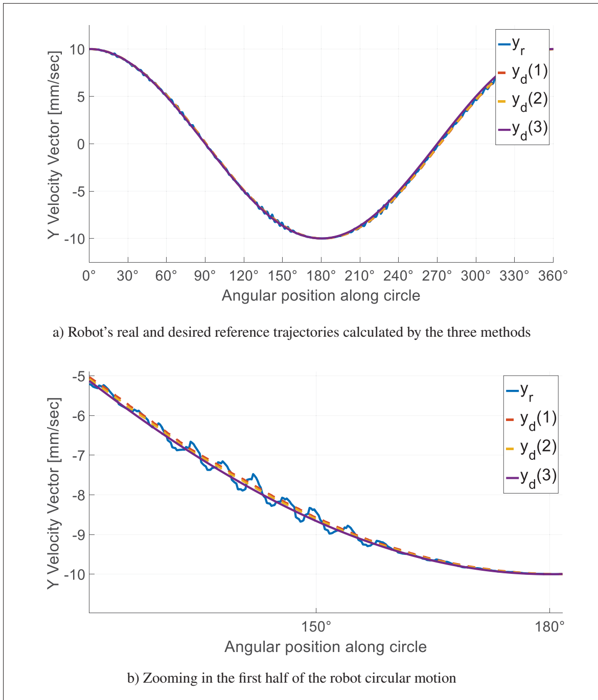
Figure 3.10 Real robot trajectory y_r , in blue color and desired reference trajectories: y_d(1) of first calculation method, in red color; y_d(2) of second calculation method, in yellow color; and y_d(3) of third calculation method, in purple color, in Y direction
