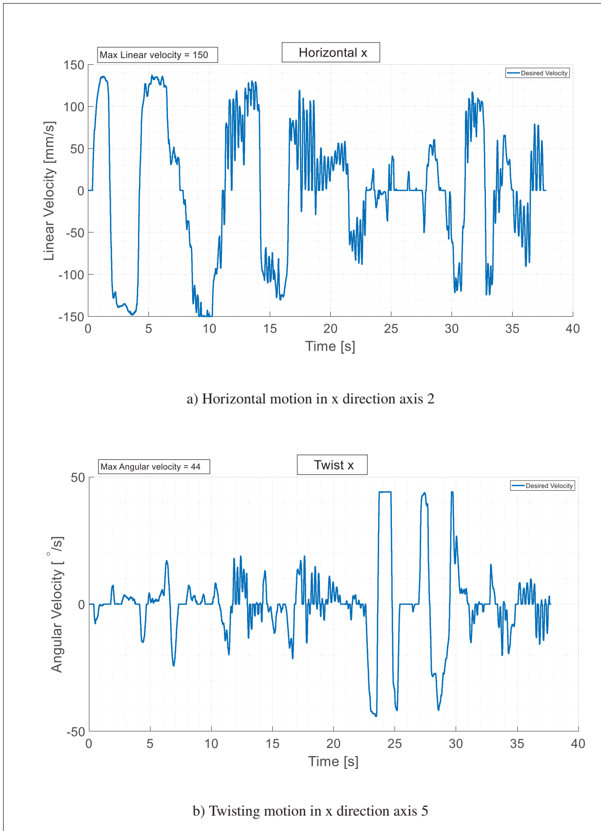
Figure 3.26 Robot's desired motion and twisting in x directions at maximum linear and angular speeds of 150 mm/s and 44 °/s, respectively
