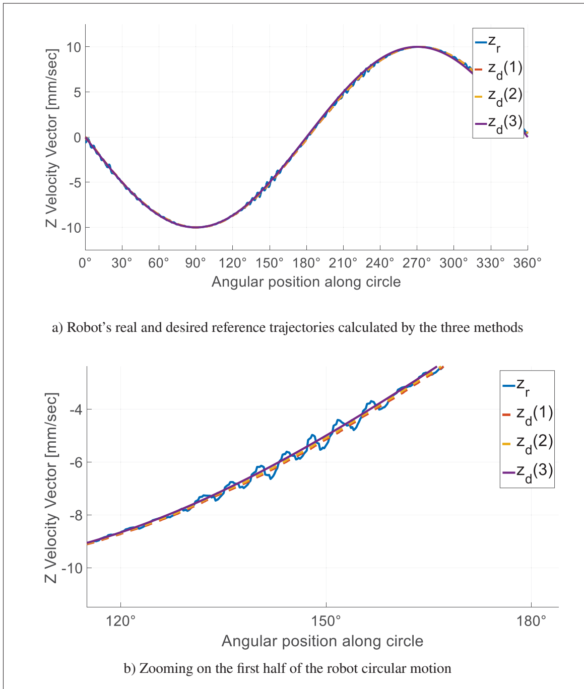
Figure 3.11 Real robot trajectory z_r , in blue color and desired reference trajectories: z_d(1) of first calculation method, in red color; z_d(2) of second calculation method, in yellow color and z_d(3) of third calculation method, in purple color, in Z direction
