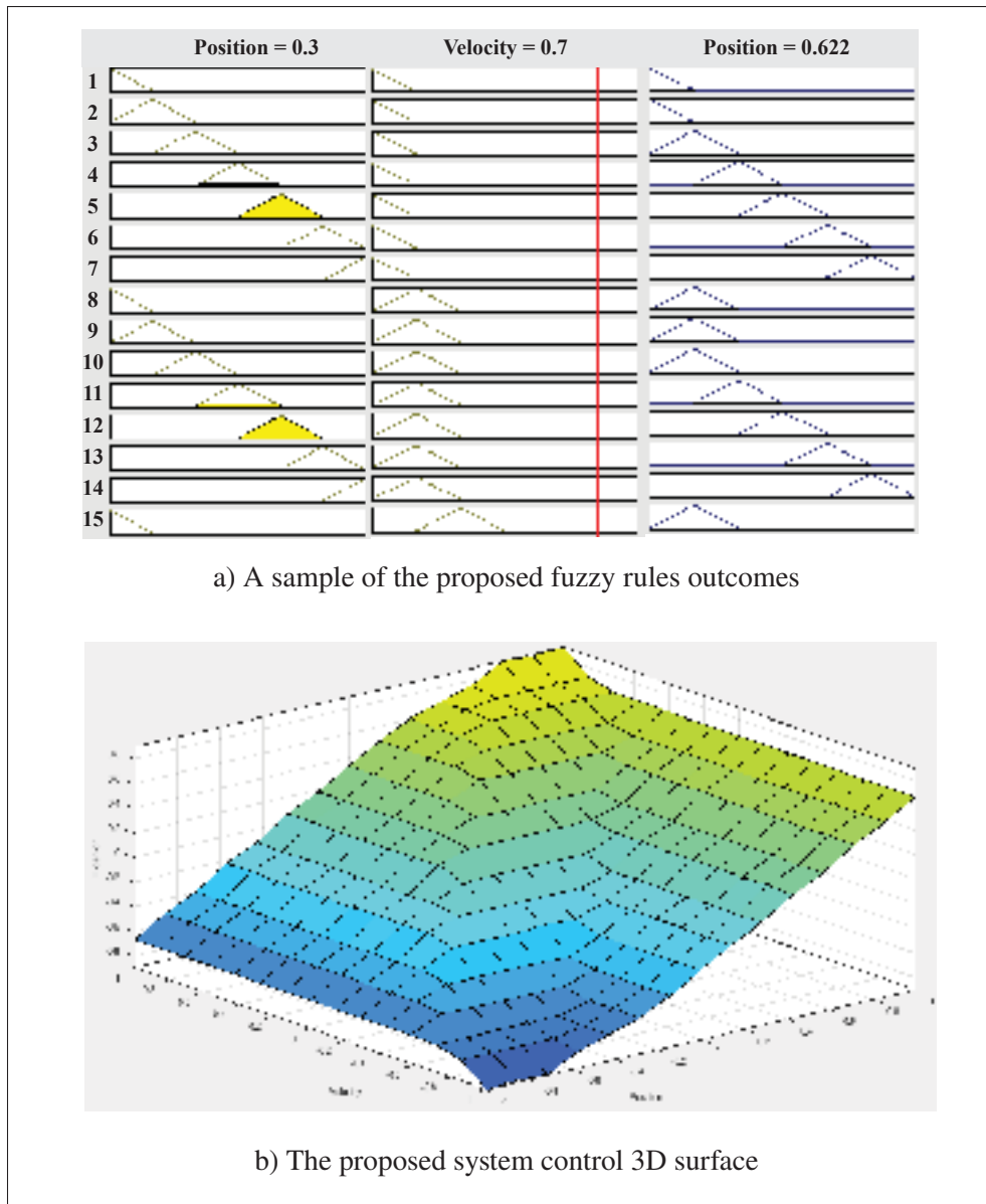
Figure 5.5 The proposed fuzzy rules outcomes and the surface exploring the relations between them using MATLAB/SIMULINK Taken from The MathWorks (2020b)
