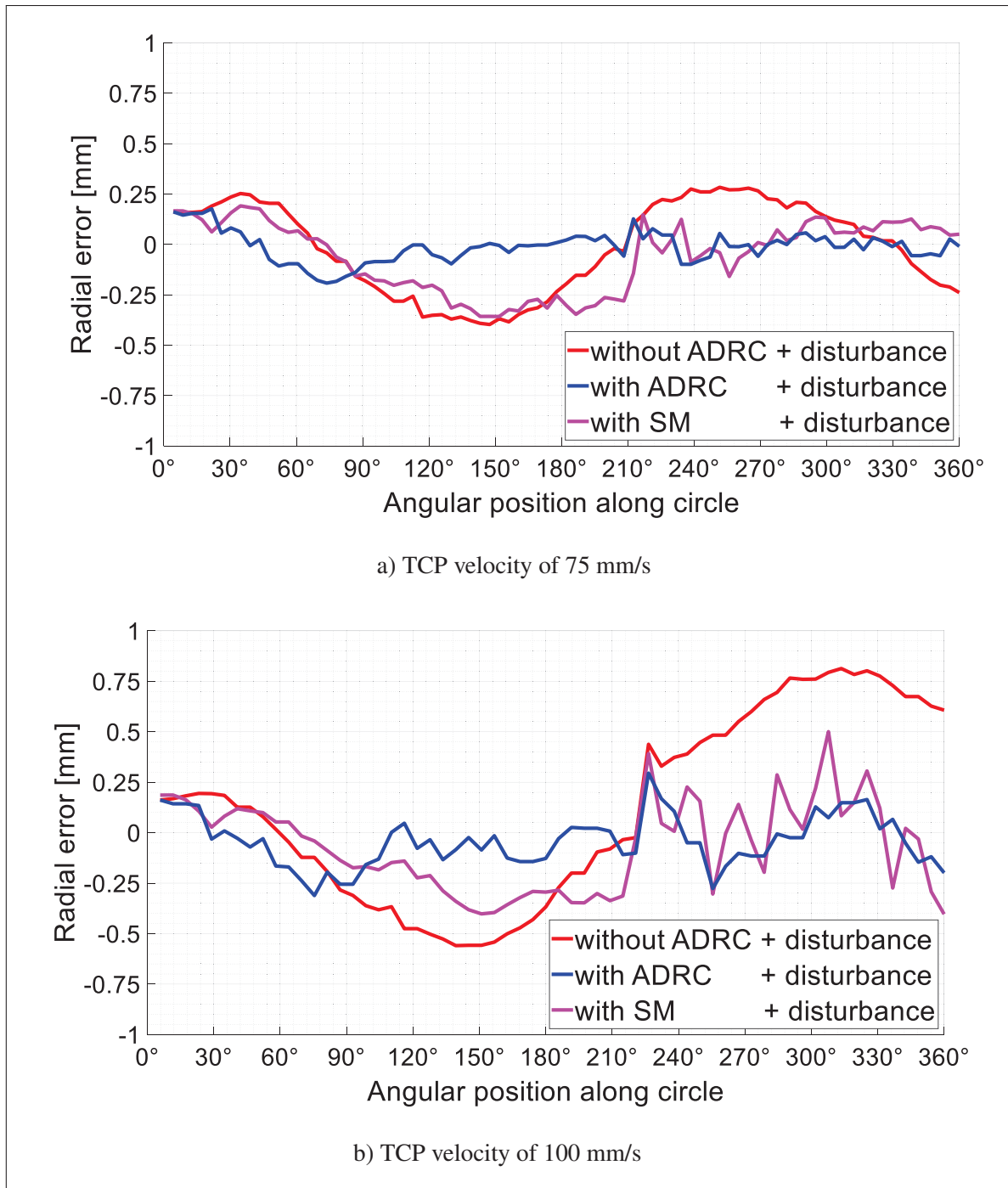
Figure 4.7 Robot's radial error measured with the ballbar at different TCP velocities, with ADRC controller, SMC controller and the sudden introduction of an extra load at angular position between 190^{\circ} to 230^{\circ} , at robot's high speeds
