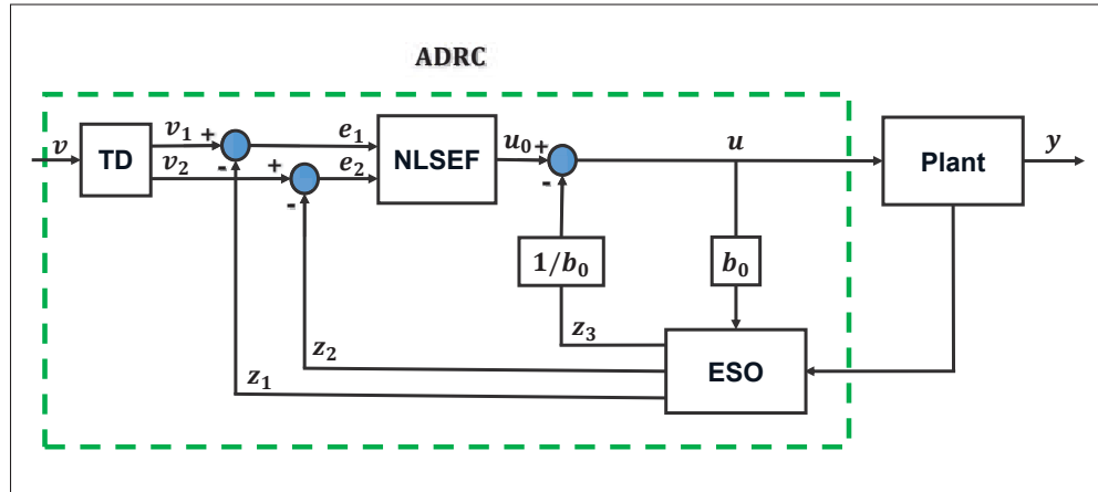
Figure 4.1 The structure of ADRC algorithm
