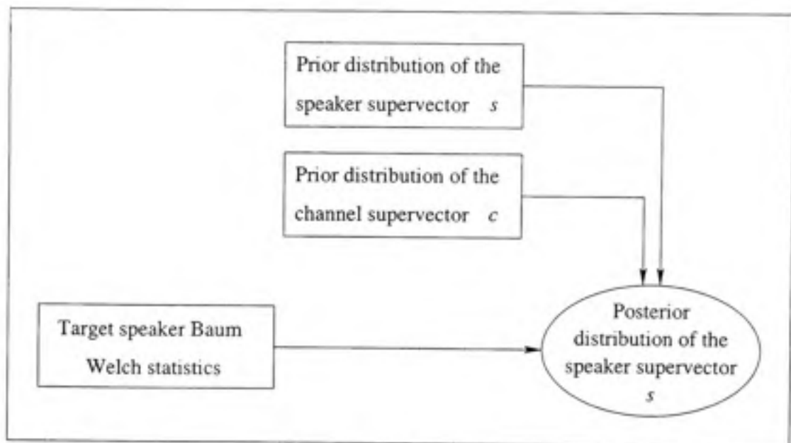
Figure 2.1 Posterior distribution of target speaker supervector.
