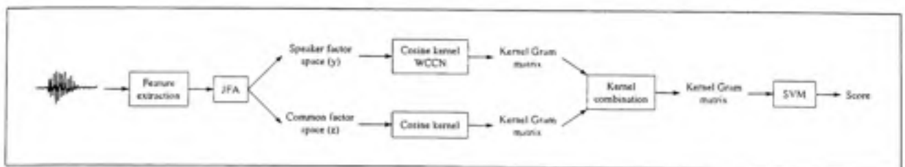
Figure 5.3 Architecture of the kernel combination system.
