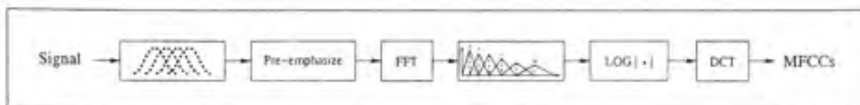
Figure 1.2 MFCC feature analysis.
