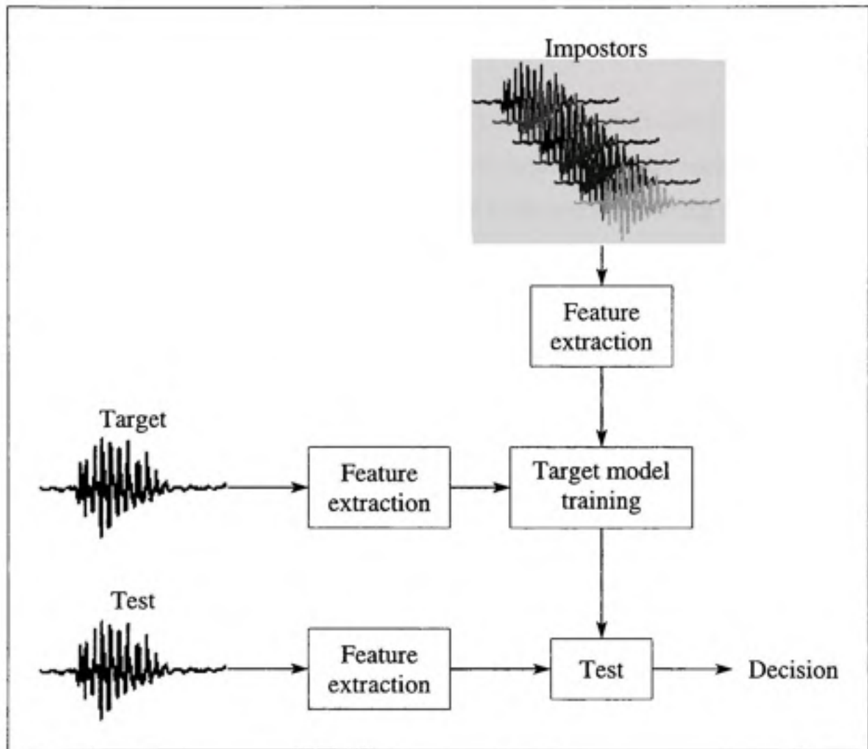
Figure 1.1 Speaker verification system.
