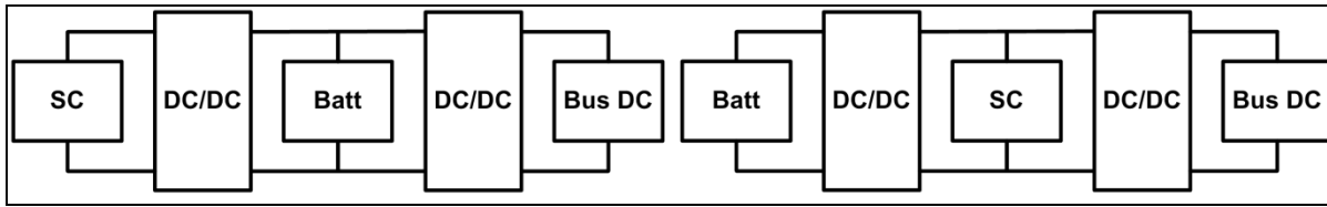
(a) Architecture active série SC/Batt/DC
