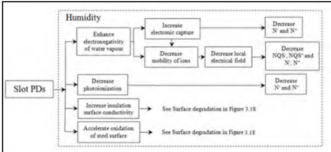
Figure 3.20 Summary of the cause and effect relationship of the influence of humidity on the slot PD activity
