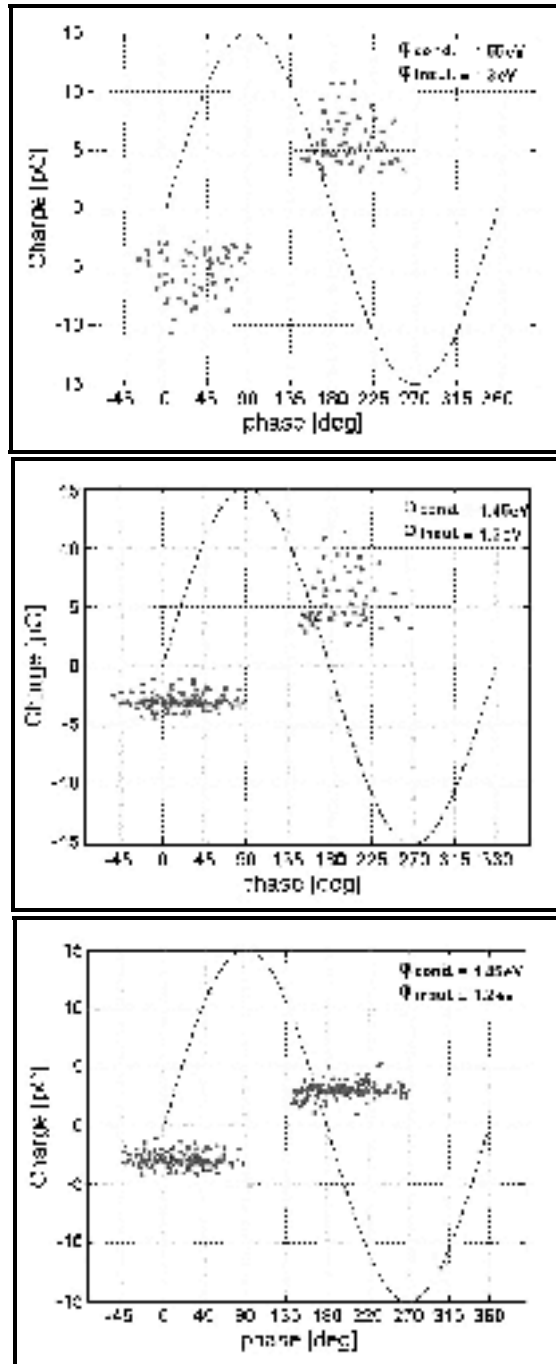
Figure 4.6 Distribution of PD events as a function of the applied voltage phase with \phi_{\text{cond}} = 1.55 \text{ eV} and \phi_{\text{insul}} = 1.3 \text{ eV} (top), \phi_{\text{cond}} = 1.45 \text{ eV} and \phi_{\text{insul}} = 1.3 \text{ eV} (middle) and \phi_{\text{cond}} = 1.45 \text{ eV} and \phi_{\text{insul}} = 1.2 \text{ eV} (bottom)
