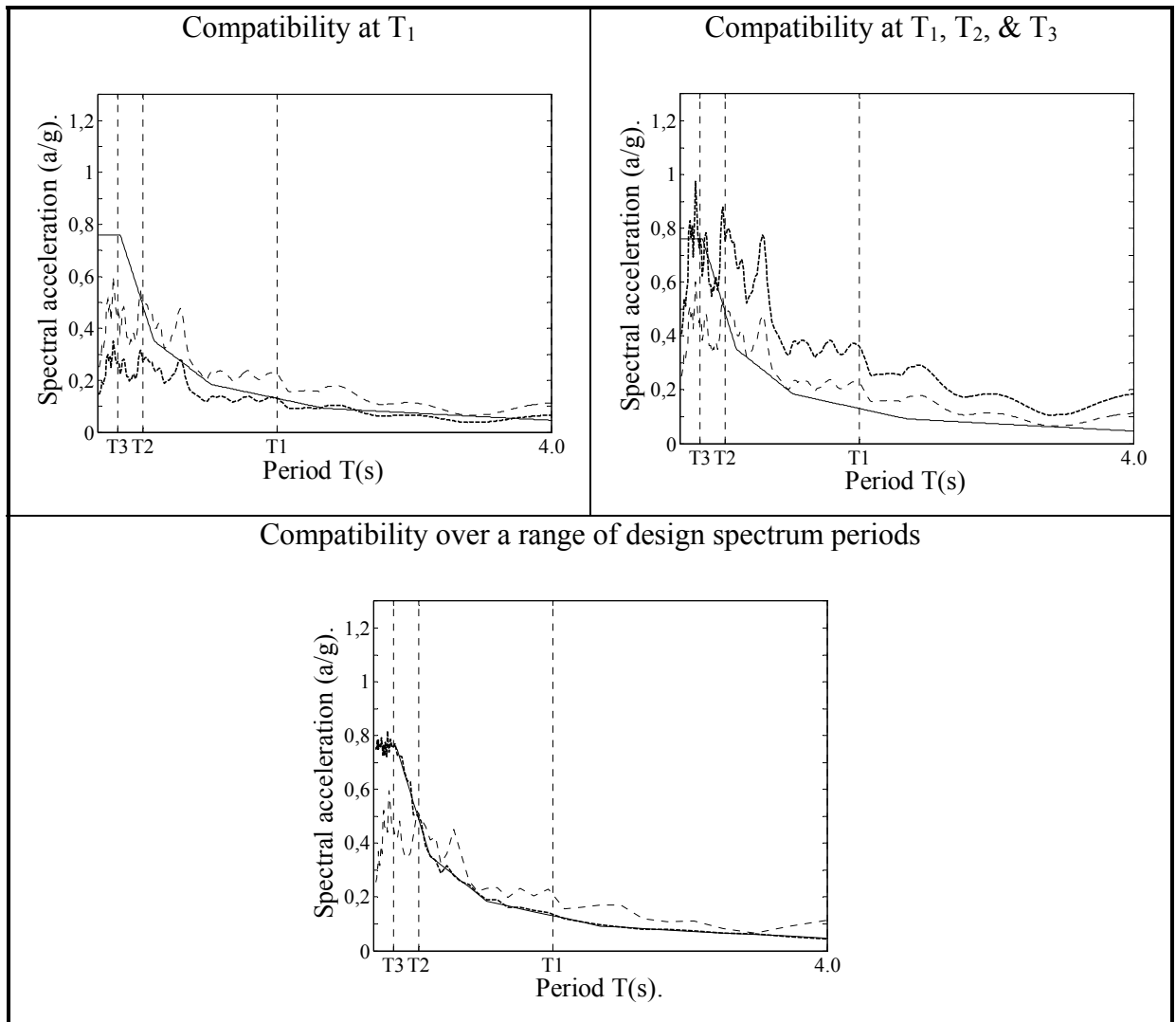
Figure 4.4 Spectrum compatibility for design - soil class A
