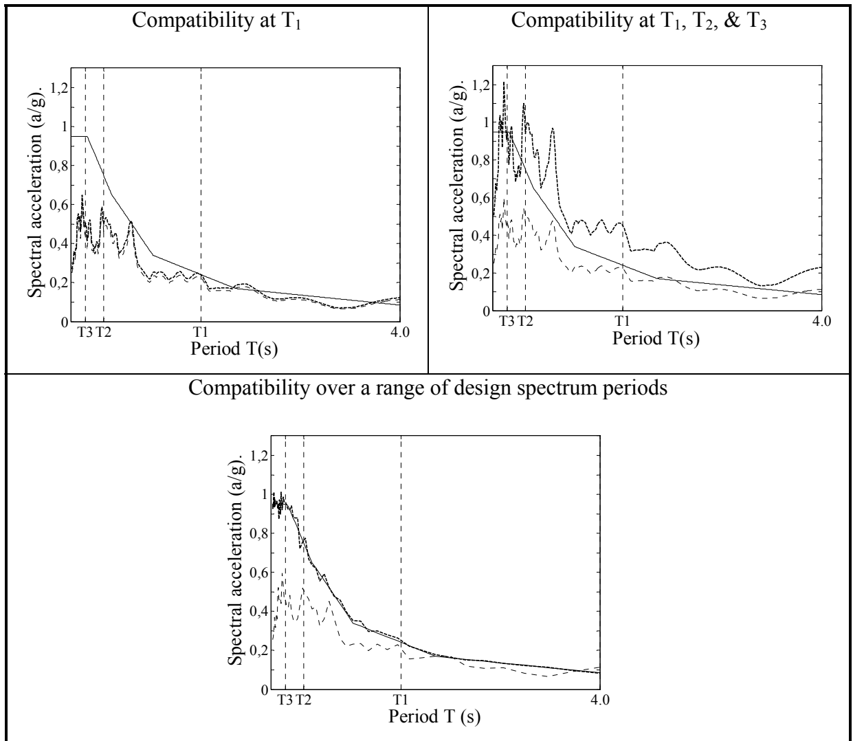
Figure 4.5 Spectrum compatibility for design - soil class C
