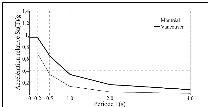
Figure 1.2 Spectres uniformes d'aléa sismique
