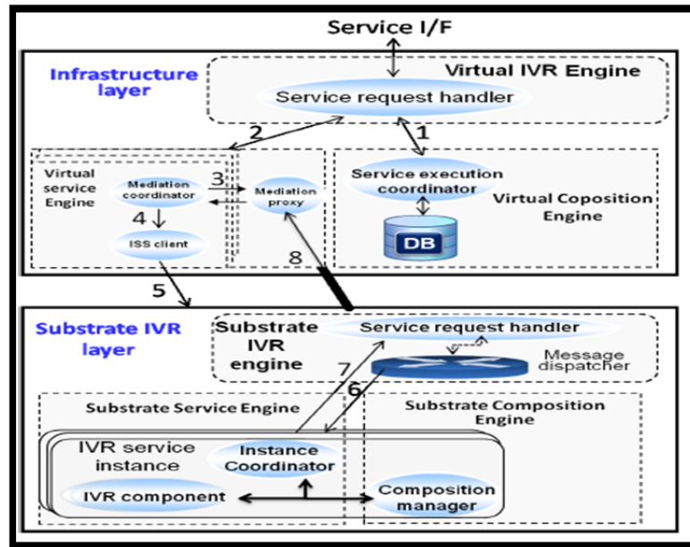
Figure 2.12 Execution Phase
