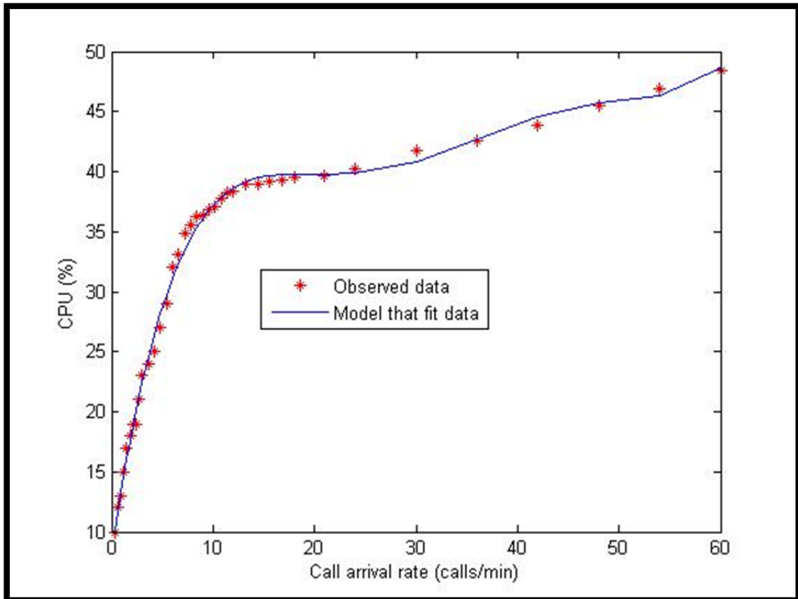
Figure 3.2 CPU Usage
