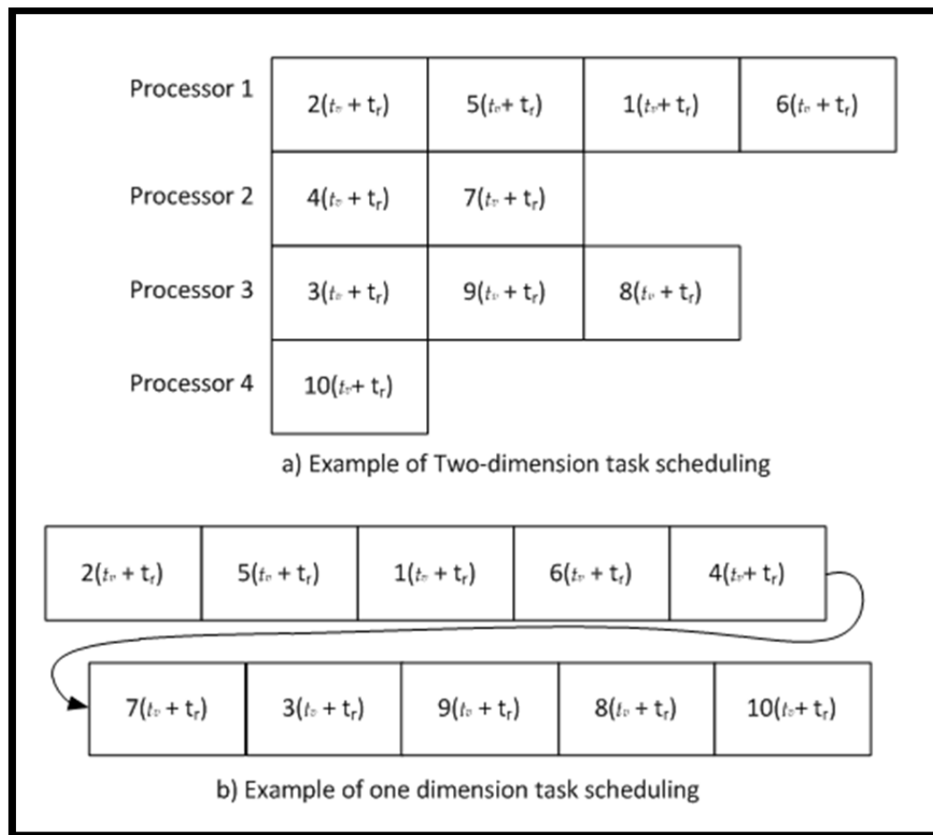
Figure 3.7 Task Scheduling
