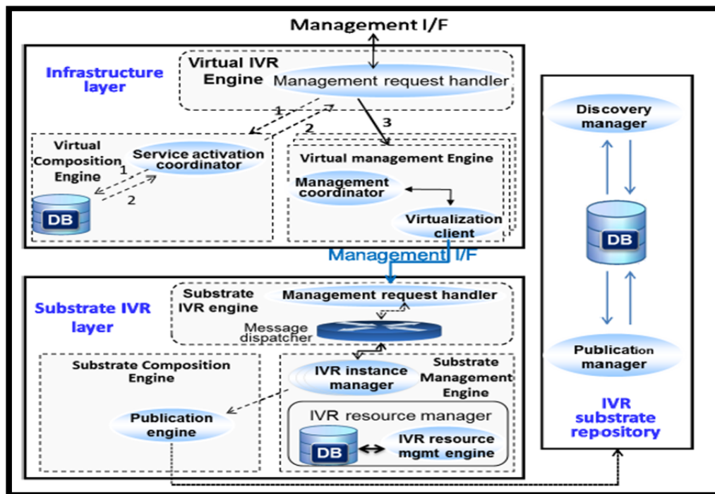
Figure 2.8 Activation Phase
