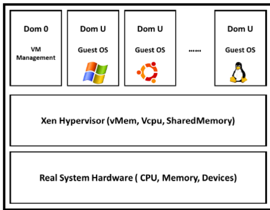
Figure 4.6 XEN Architecture
