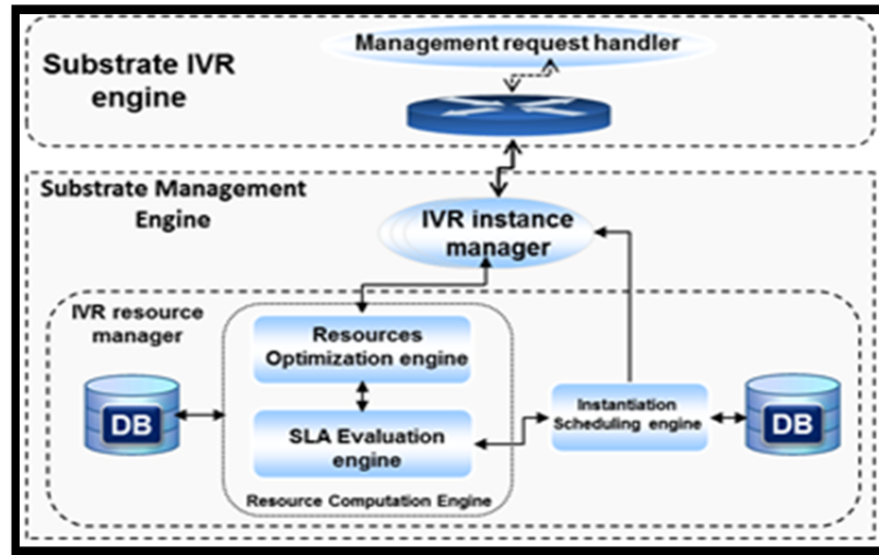
Figure 2.10 Management Phase
