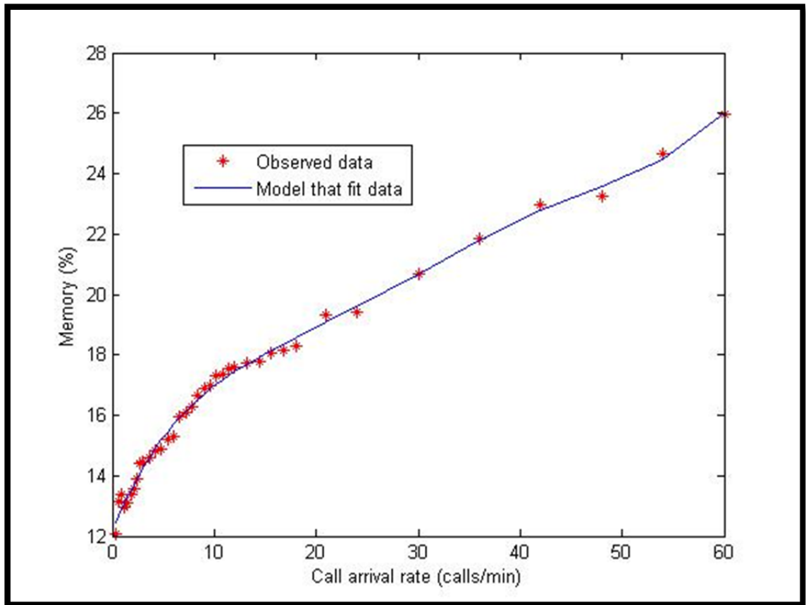
Figure 3.3 Memory Usage
