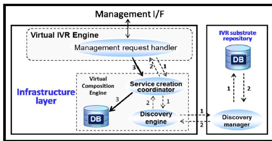
Figure 2.5 Creation Phase
