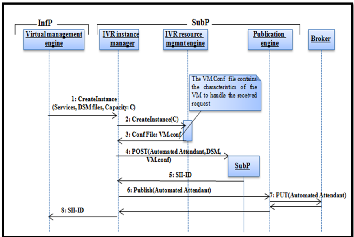
Figure 2.11 Service Management
