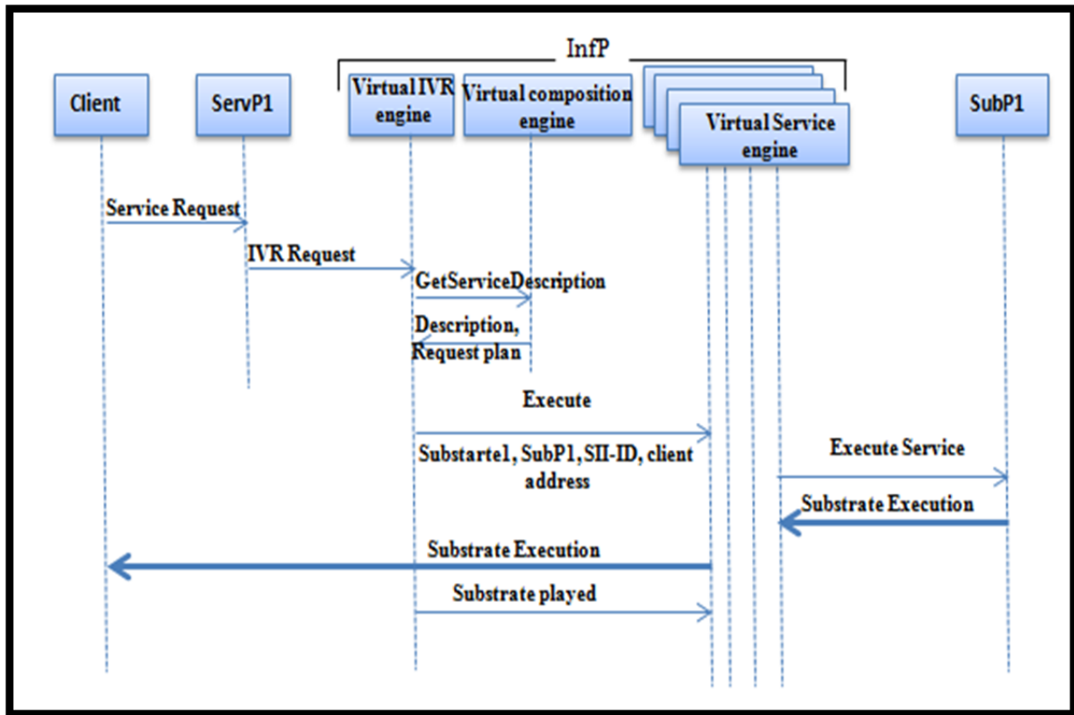
Figure 2.13 Service Execution
