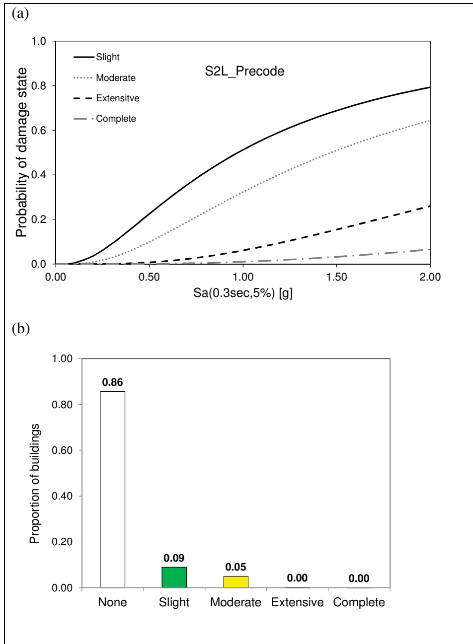
Figure-A V-3 Illustration of damage assessment using the procedure in this study: (a) fragility functions for S2L-Precode building class and (b) the predicted damage proportions at S_a(0.3\text{sec}, 5\%) = 0.38\text{g} .
