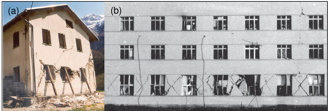
Figure 1.9 Photographs illustrating typical diagonal cracking damage for: (a) a stone masonry buildings and (b) a brick masonry building Taken from Lutman and Tomazevic (2002)
