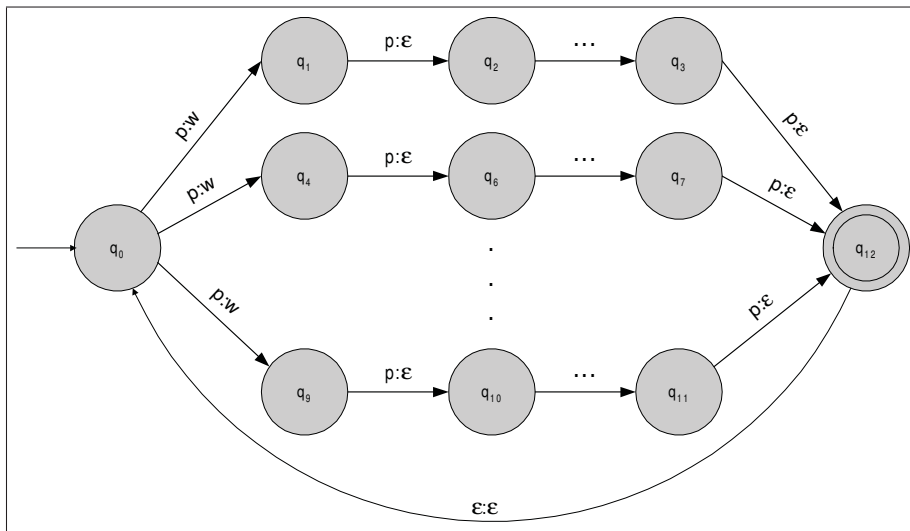
Figure 3.6 Dictionary transducer
