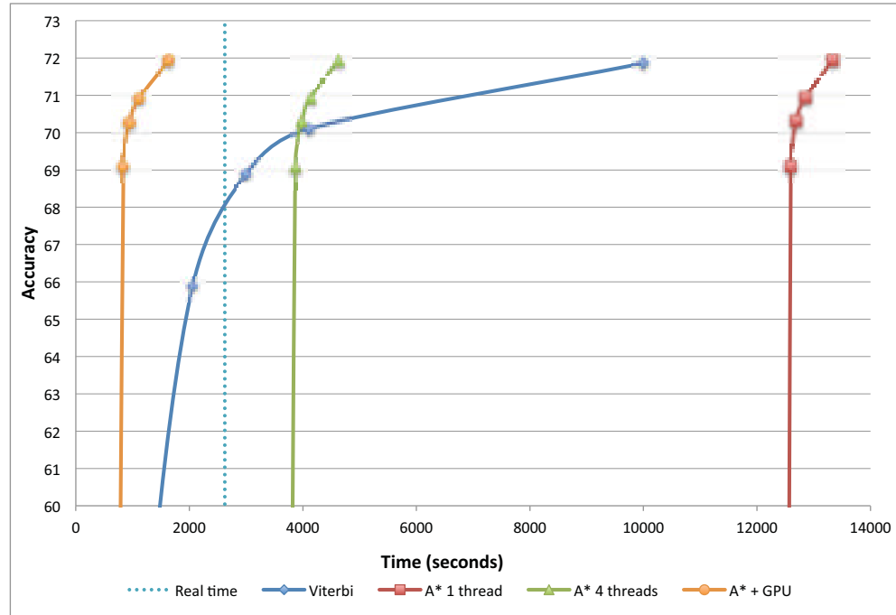
Figure 4.2 A* with GPU decoder accuracy vs execution time.
