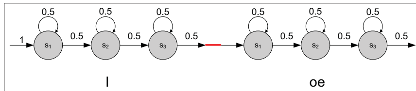
Figure 0.4 Simplified model for the word "le".
