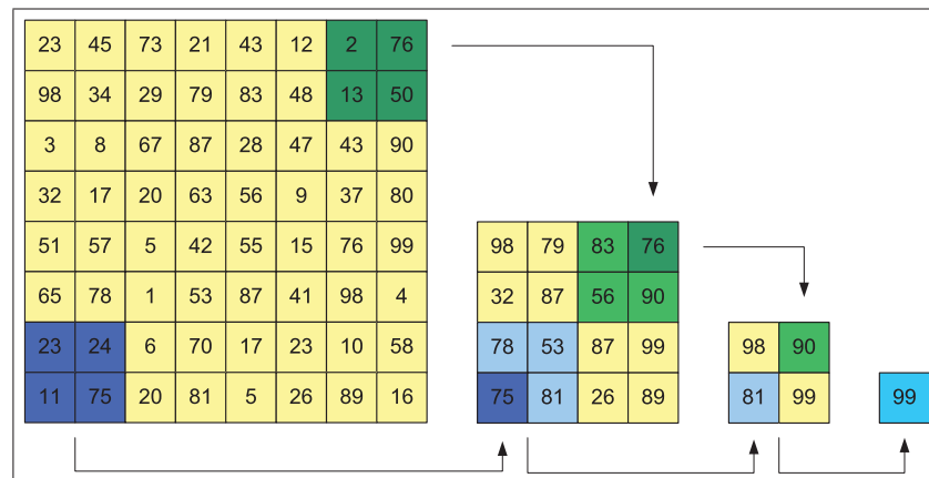
Figure 2.3 Reduction algorithm Image is from Harris (2005)).
