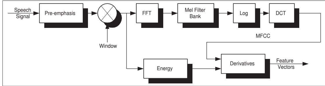
Figure 1.2 MFCC Processing
