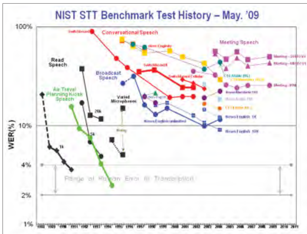
Figure 0.1 NIST STT benchmark test history
