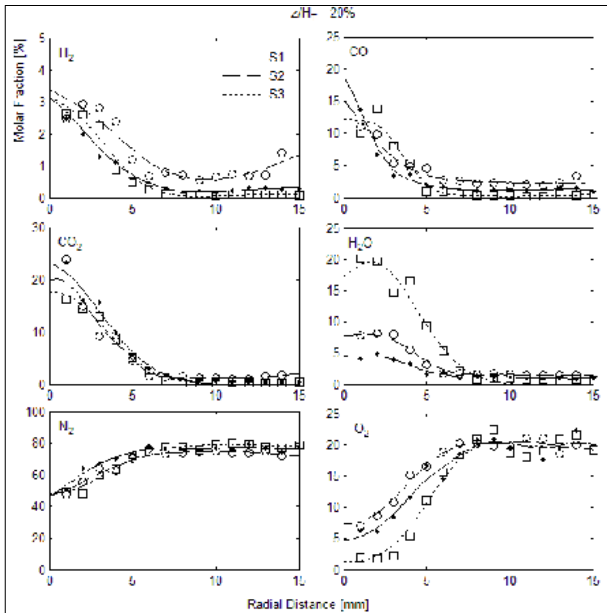
Figure 3.5 Radial profiles of species concentrations for S1, S2 and S3 fuels, measured at 20% of flame height ( \bullet = S1: 25H 2 /50CO/25CO 2 , \circ = S2: 37.5H 2 /37.5CO/25CO 2 , \square = S3: 50H 2 /25CO/25CO 2 )
