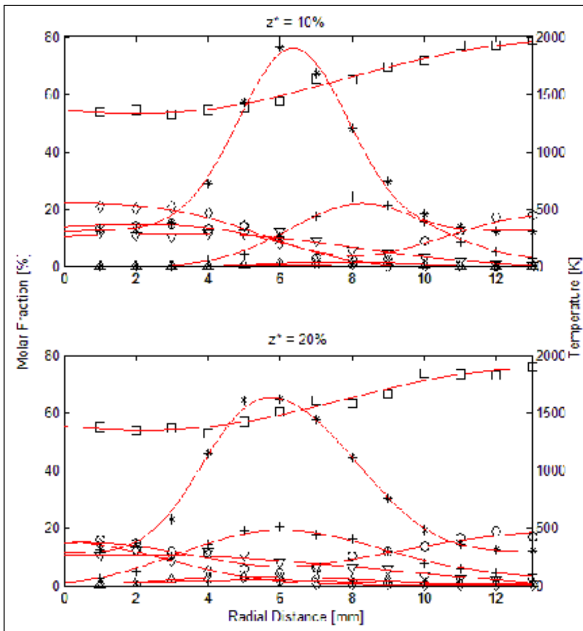
Figure 3.2 Radial profiles of temperature and species concentrations of the B1 flame at z^*=10\% and 20\% ( \times =H 2 , \Delta =CO, + =H 2 O, \nabla =CO 2 , \square =N 2 , \circ =O 2 , * =Temp)
