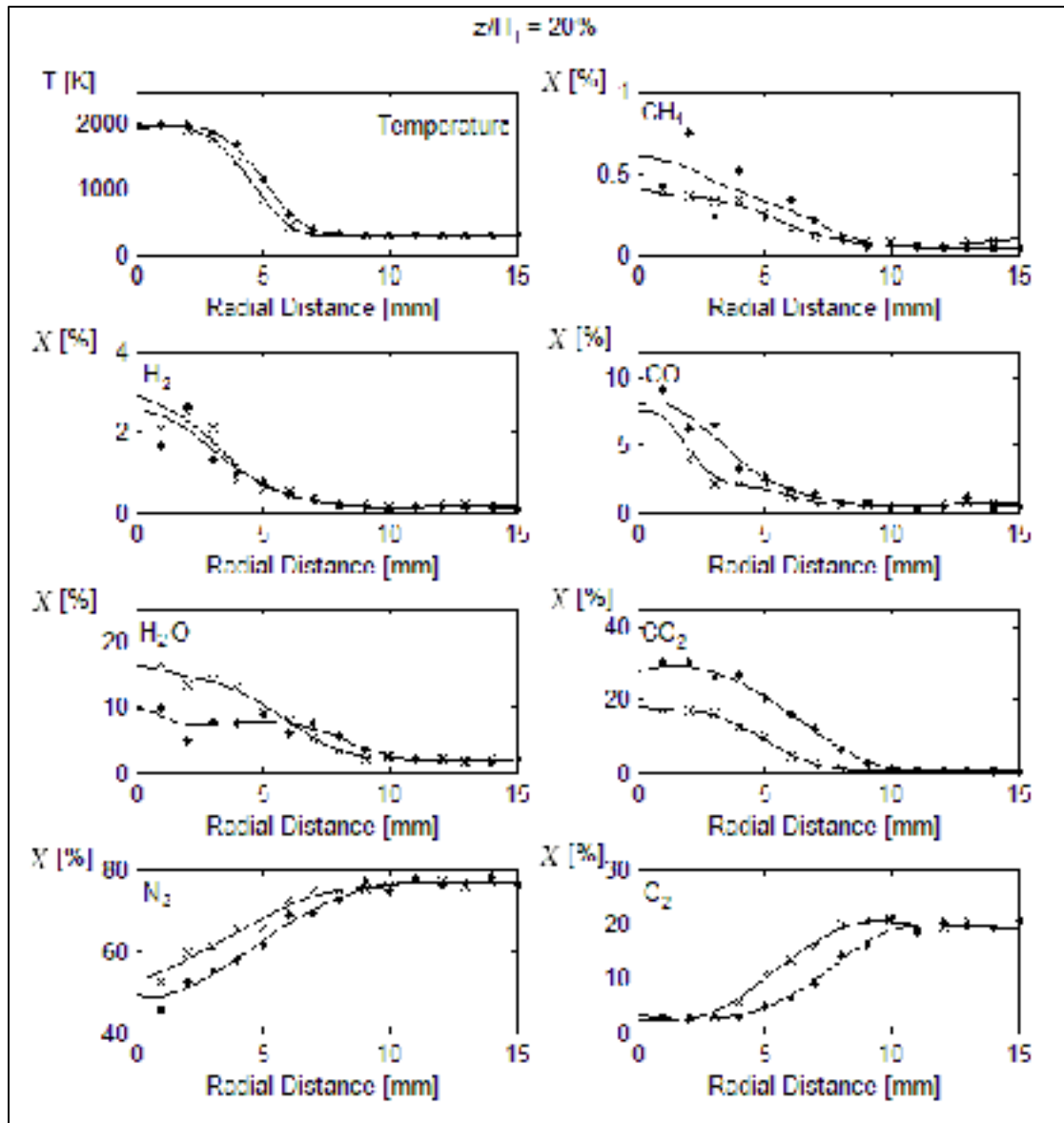
Figure 3.9 Comparison of species concentrations and temperature for S5 and S6 fuel measured at z/H_1=20\% ( \bullet = S5: 37.5\text{H}_2/37.5\text{CO}/5\text{CH}_4/25\text{CO}_2 , \times = S6: 50\text{H}_2/25\text{CO}/5\text{CH}_4/20\text{CO}_2 )
