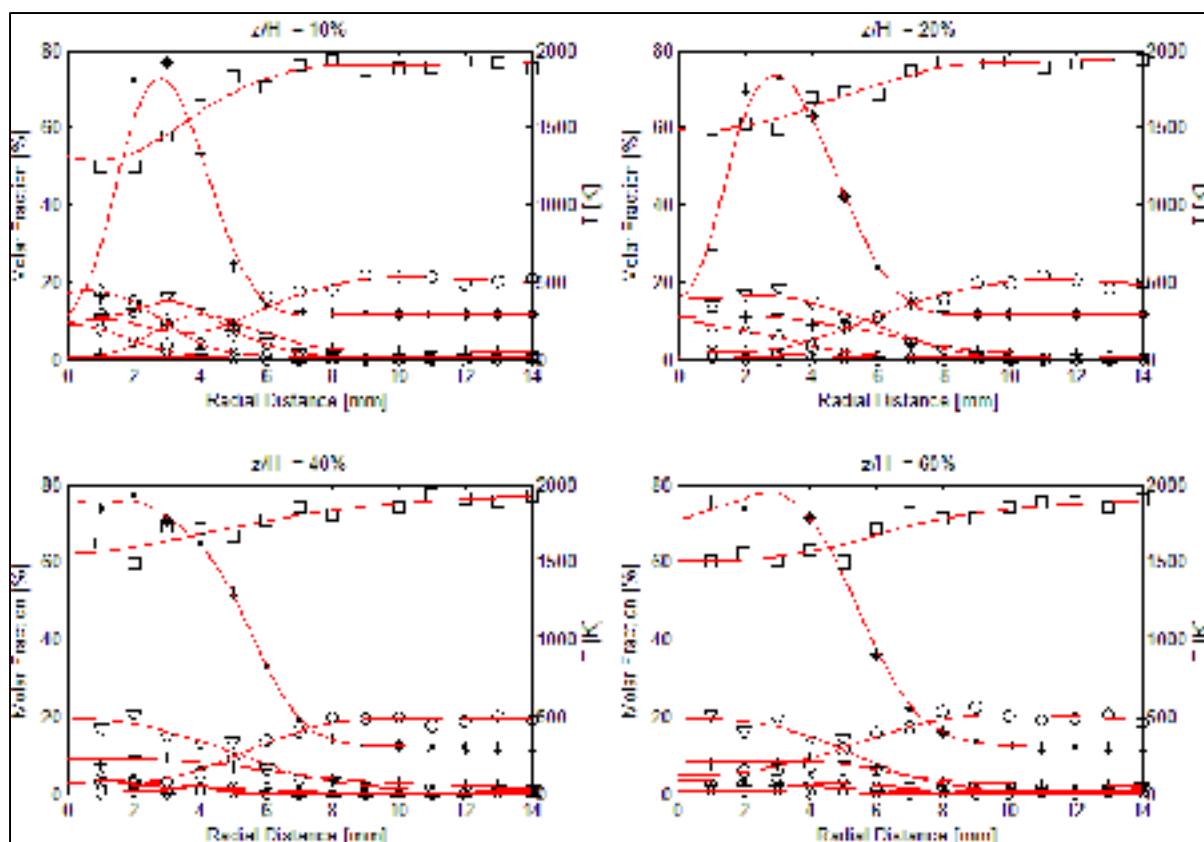
Figure-A I-9 Radial profile of S5M25 flame ( \times = \text{H}_2 , \Delta = \text{CO} , \diamond = \text{CH}_4 , + = \text{H}_2\text{O} , \nabla = \text{CO}_2 , \square = \text{N}_2 , \circ = \text{O}_2 , * =Temp)
