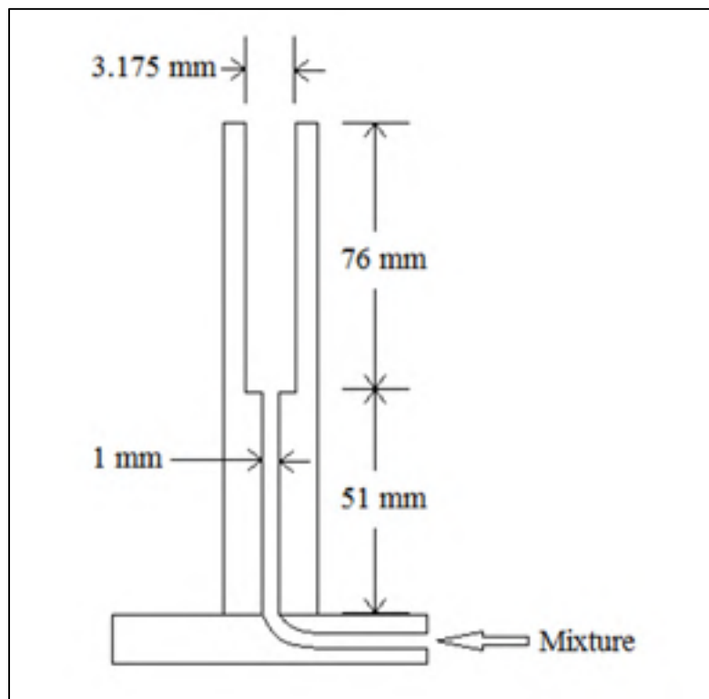
Figure 2.1 Dimensions of 3.175 mm inner diameter burner
