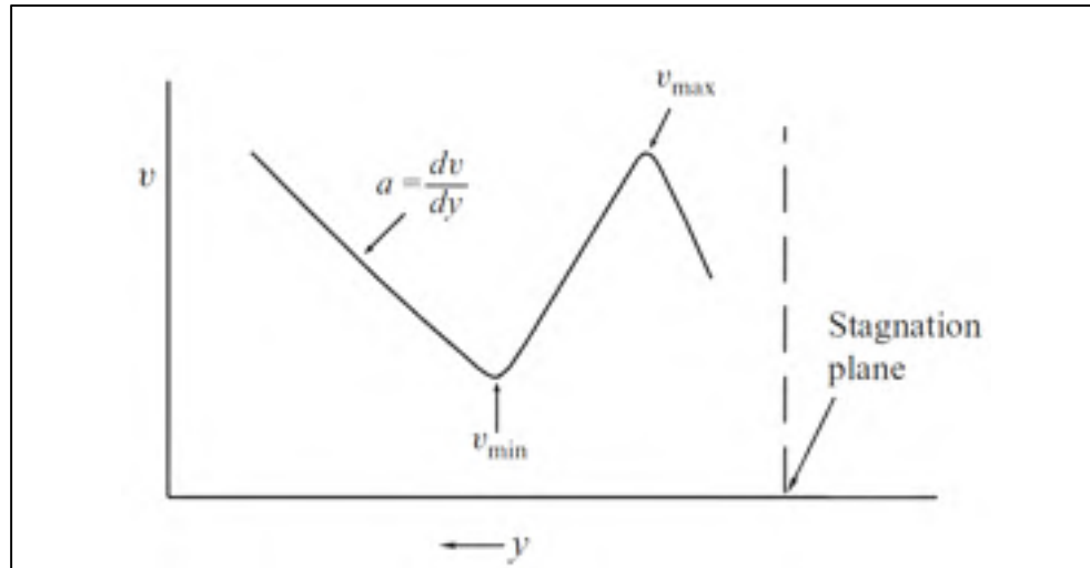
Figure 1.11 Axial profile illustrating the normal velocity of the gas flow with respect to the distance from the stagnation plane Taken from C.K. Law, Combustion Physics , Cambridge press (2006, p. 272)
