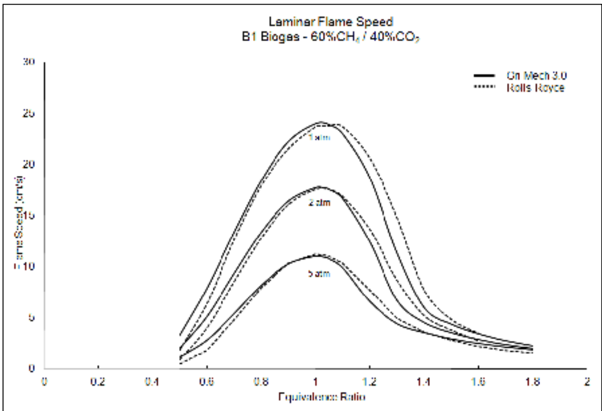
Figure-A IV- 1 Laminar flame speed with respect to equivalence ratio of B1 flame
