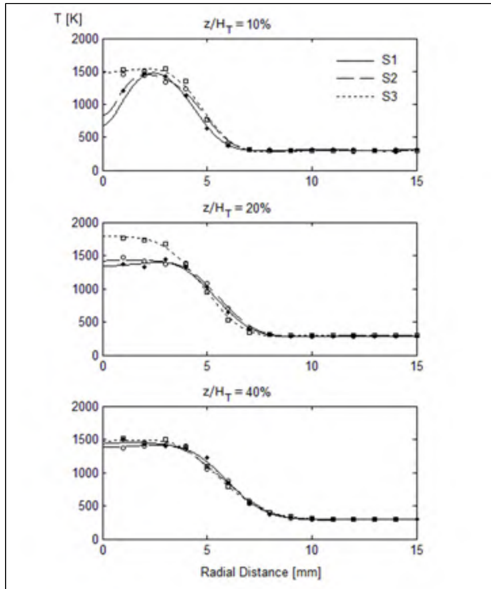
Figure 3.4 Temperature profiles of S1, S2 and S3 flames at various flame elevations ( \bullet = S1: 25\text{H}_2/50\text{CO}/25\text{CO}_2 , \circ = S2: 37.5\text{H}_2/37.5\text{CO}/25\text{CO}_2 , \square = S3: 50\text{H}_2/25\text{CO}/25\text{CO}_2 )
