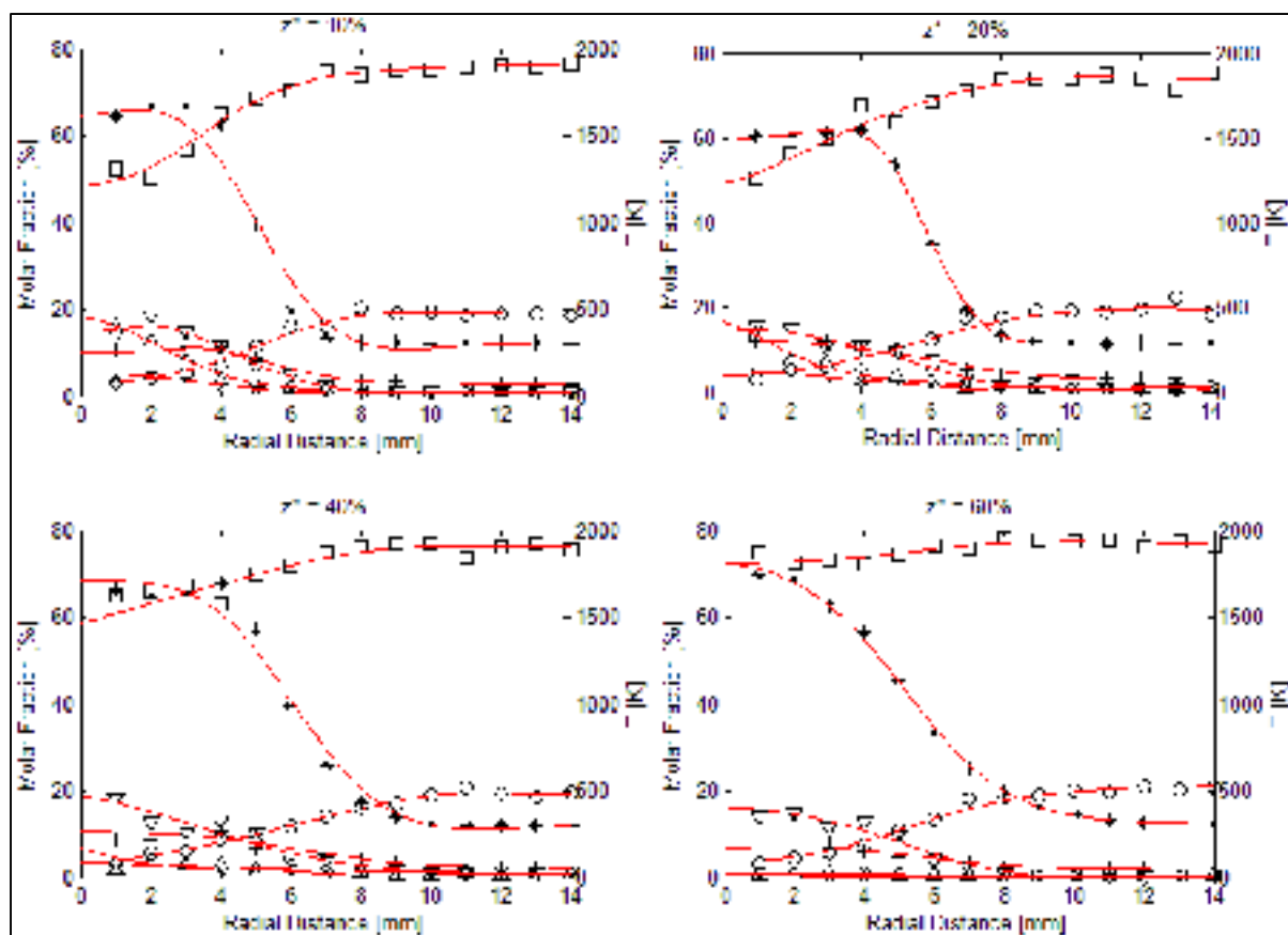
Figure-A I-5 Radial profile of S14 flame ( \times=H_2 , \Delta=CO , + = H_2O , \nabla=CO_2 , \square=N_2 , \circ=O_2 , *=Temp )
