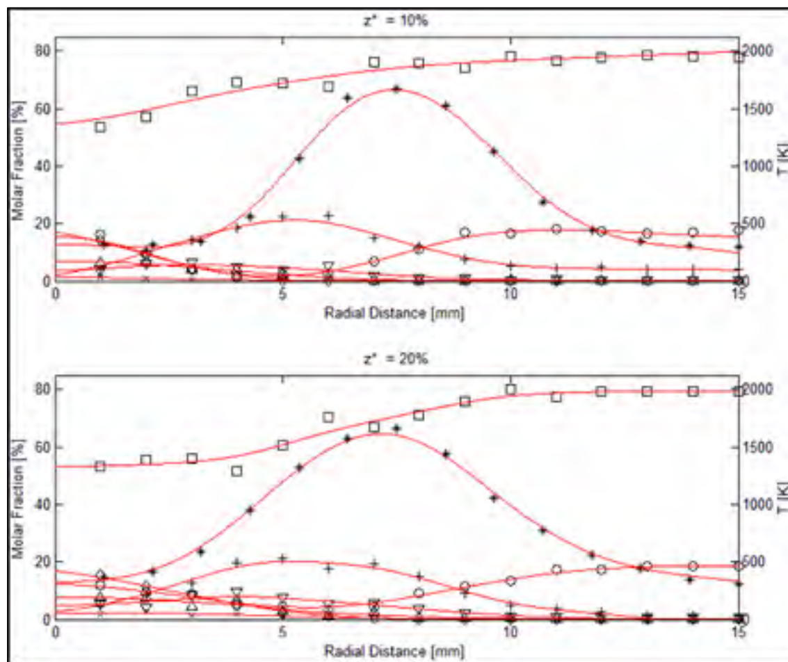
Figure 3.10 Radial profile of species concentration and flame temperature of S5M50 flame ( \times =H 2 , \Delta =CO, \diamond =CH 4 , + =H 2 O, \nabla =CO 2 , \square =N 2 , \circ =O 2 , * =Temp)
