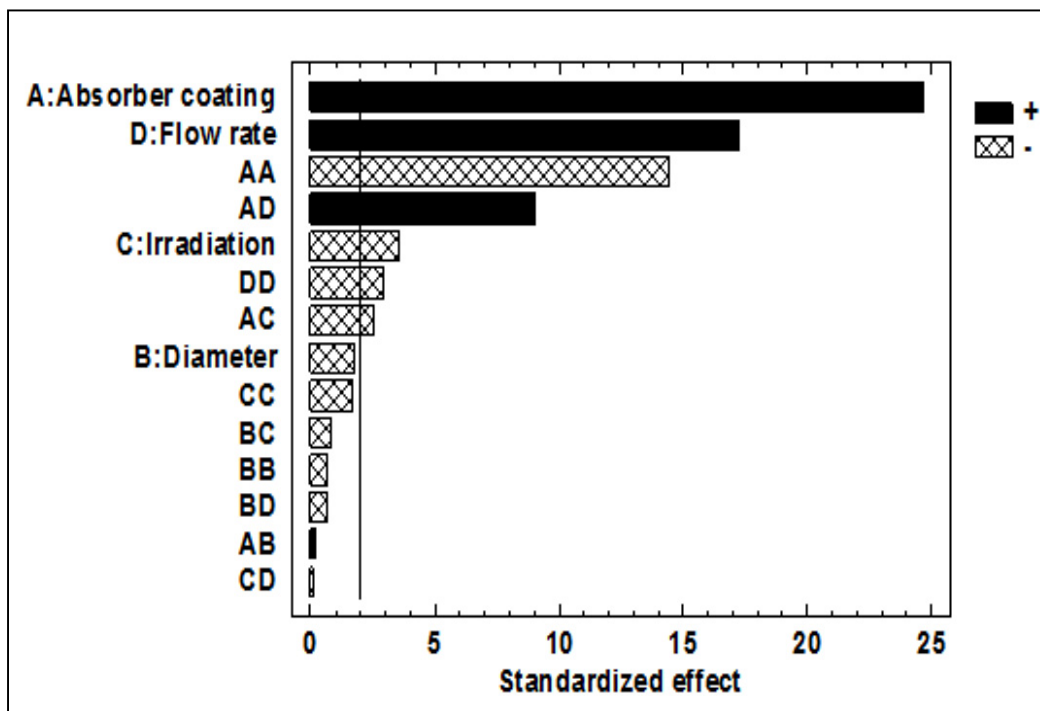
Figure 2.5 Standardized Pareto chart for efficiency
