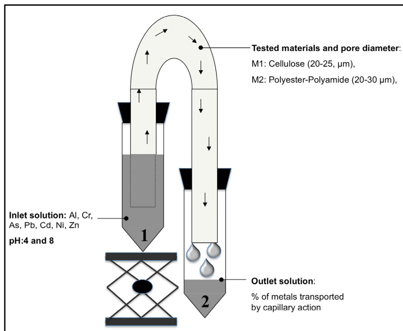
Figure 2.1 Capillary siphon
