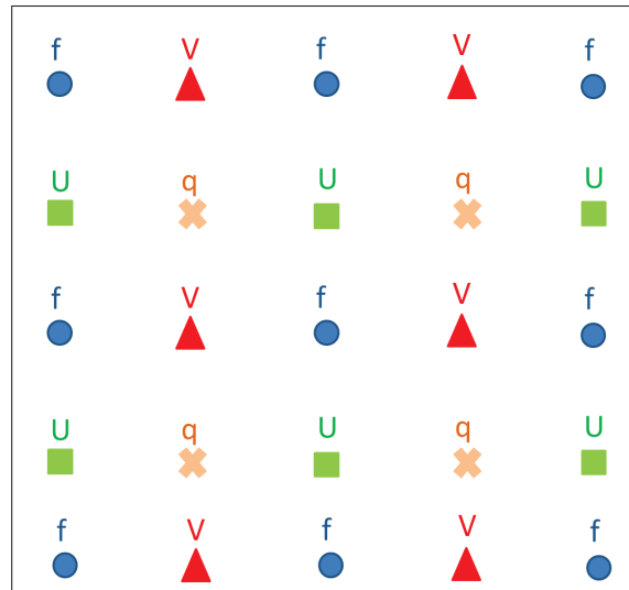
Figure 4.2 Grille de type Arakawa C
