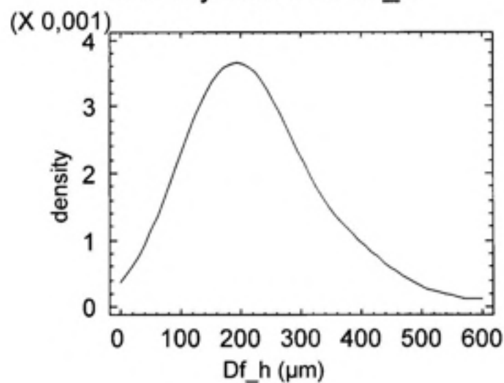
Density Trace for Df_h
