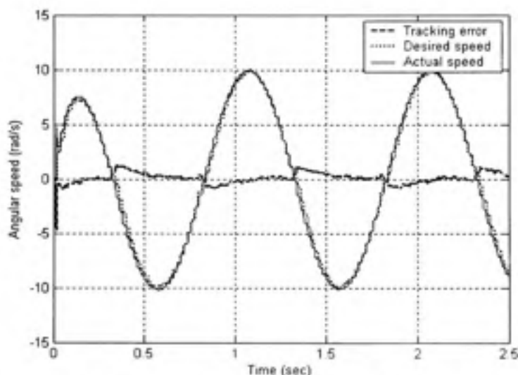
Figure 2.8 Experimental velocity and tracking error for Backstepping controller with maximum load applied on the hydraulic actuator.
