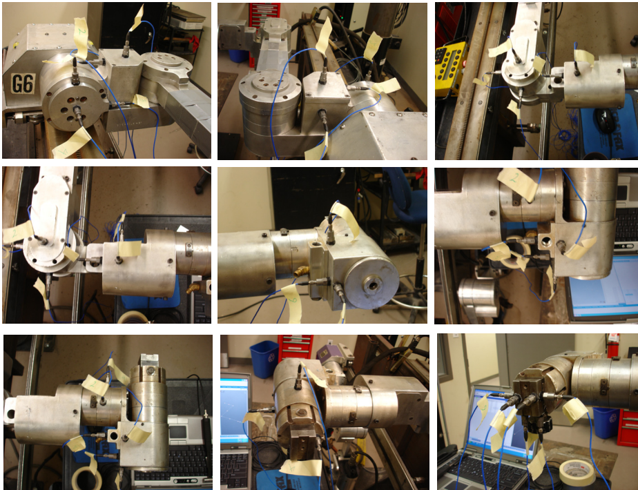
(b) Attachment of accelerometers on the robot structure
