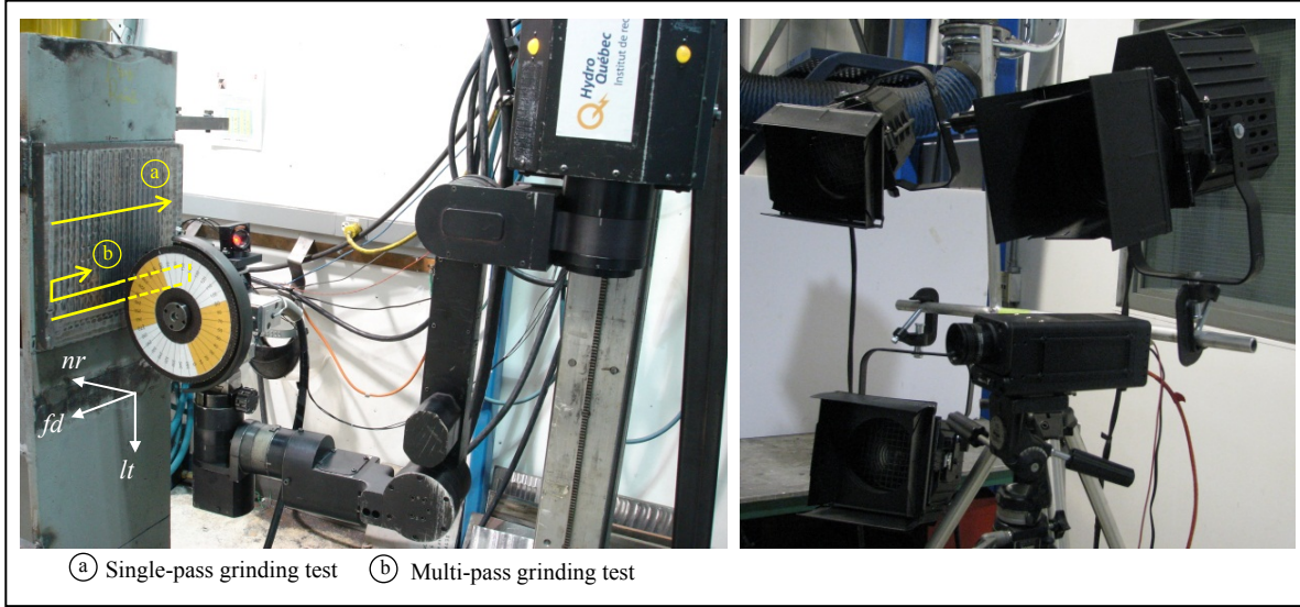
Figure 3.10 Robotic grinding test rig with high-speed camera and lighting
