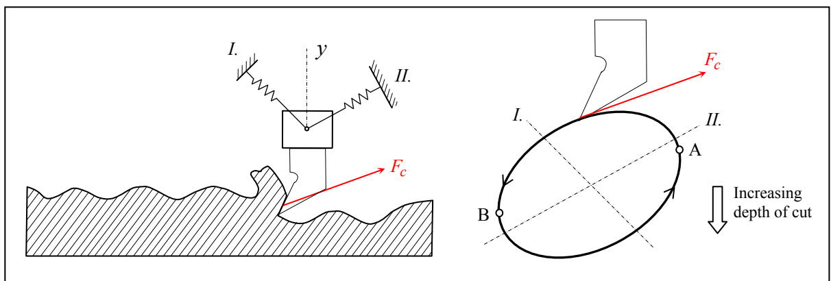
Figure 1.4 Mode-coupling instability in machining adapted from (Tlustý and Polacek, 1963)
