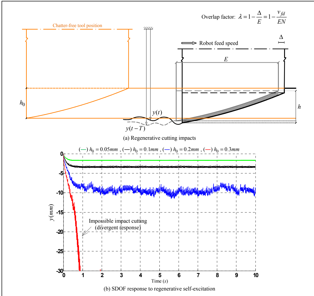
Figure 4.7 Unstable impact cutting
