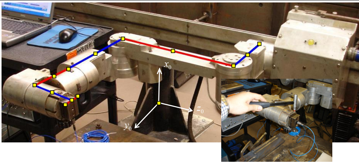
(a) Vertical excitation at the end-effector
