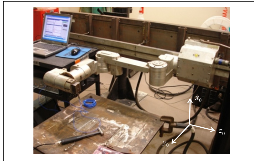
Figure 5.3 Configuration of SCOMPI for modal testing experiment
