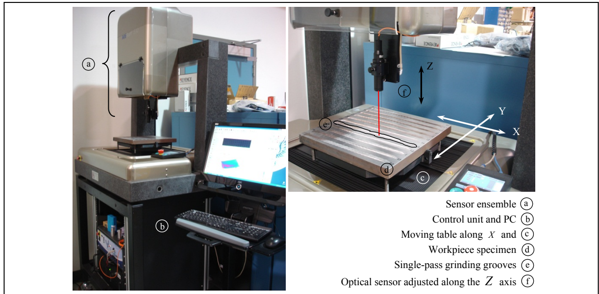
Figure 3.12 AltiSurf 530 machine
