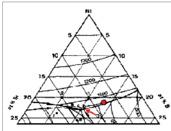
Figure 3.7 Part of the solidus surface of the ternary diagram ; red arrow points on the ternary eutectic (point b) ; red point indicates the approximate position of BNi-2 alloy, assuming that Cr and Fe are equivalent to Ni. Diagram from Lebaili
