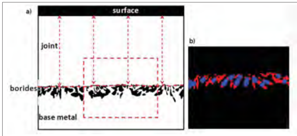
Figure 3.1 Quantitative analysis of microstructures : a) Schematic representation of the different layers of a brazed sample, along with the method used to measure joint thickness and a frame used for boride size and amount measurement ; image is not to scale ; b) image interrupted at a given step of the iterative process used to measure boride mean size (see section above) ; initial borides in red and blue, surface still present at this opening step in blue.
