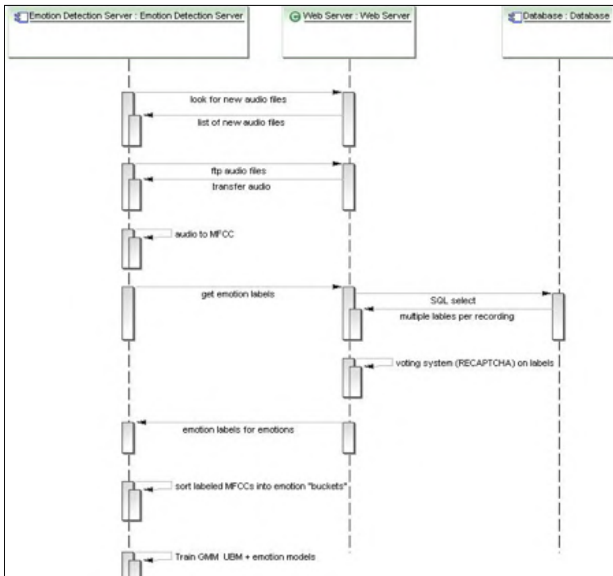
Figure 132 Emotion Detector Training Sequence Diagram
