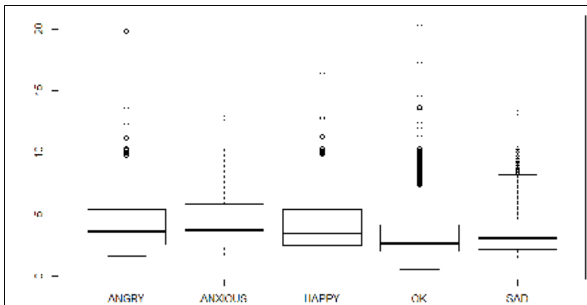
Figure 201 Predicted Probabilities of Length-of-Speech versus Emotion
