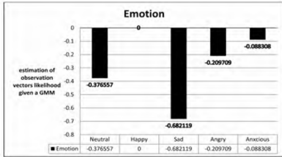
Figure 80 Real-Time Acoustic Emotion Classifier determines Happy
