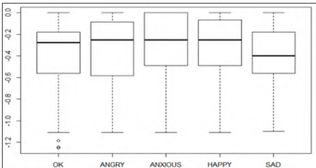
Figure 216 Predicted Probabilities of Confusability versus emotion
