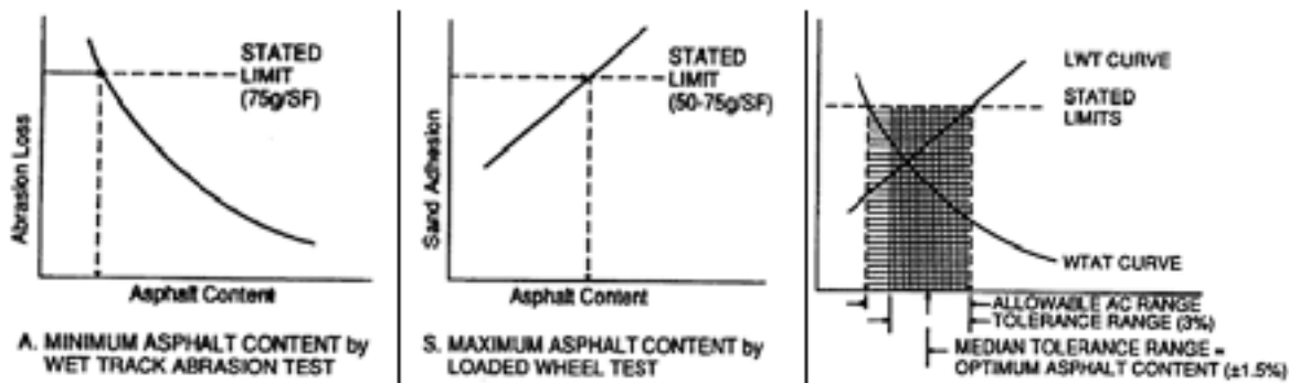
Figure 3.1 Graphical Determination of Optimum Asphalt Content Extracted from ISSA (2004, p. 13)
