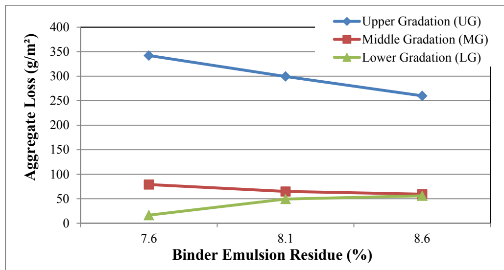
Figure 4.4 Plot of raw data for WTAT 1-Hour Soaked
