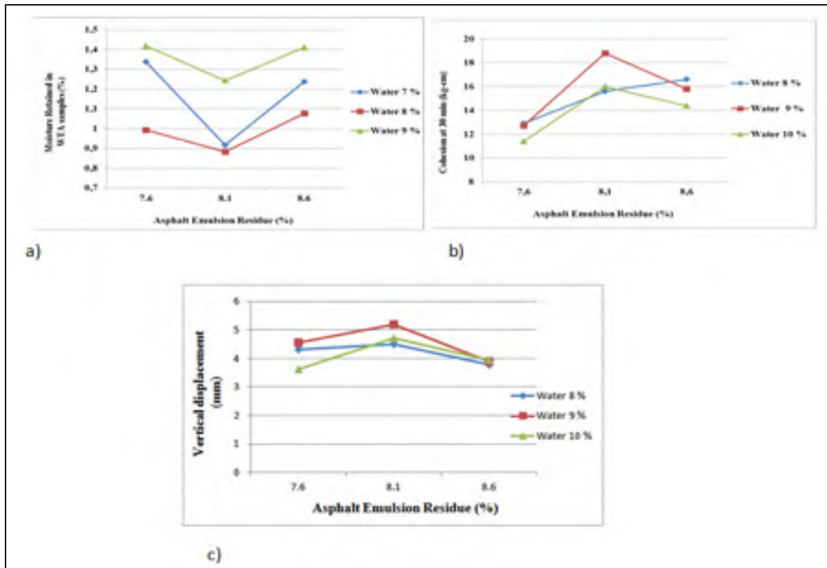
Figure 3.3 Effect of asphalt emulsion and water contents on: a) retained moisture (WTAT samples), b) Cohesion test at 30 min, and c) vertical displacement test
