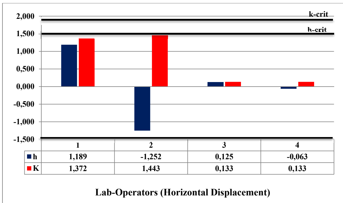
Figure 5.9 Lateral displacement test results, plot of h and k consistency statistics versus material type combinations
