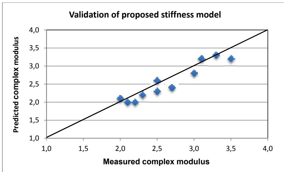
Figure 6.15 Correlation between measured and predicted complex modulus
