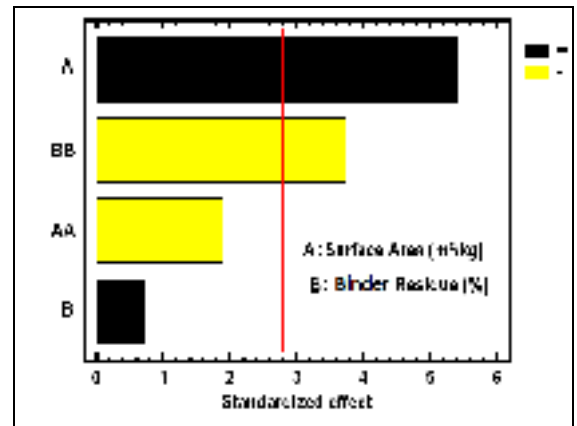
Figure 4.15. Pareto chart (Cohesion test at 60 min)
