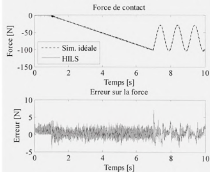
Figure 5.19 Force de contact de la simulation sans application de la contrainte (PID).
