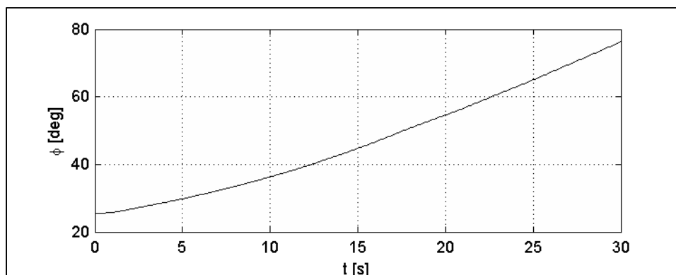
Figure 2.18 – Mode spirale instable (ID 805)
