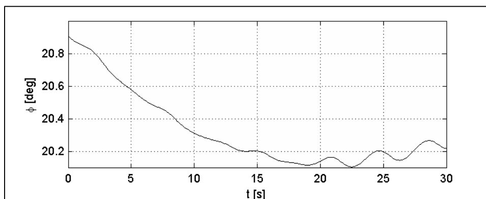
Figure 2.19 – Mode spirale neutre (ID 880)
