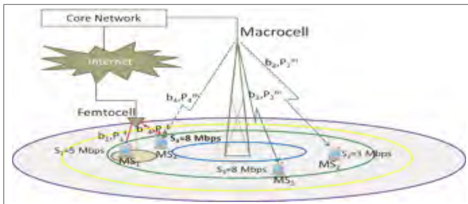
Figure 2.1 A OFDMA macro-femtocell network with four mobile users
