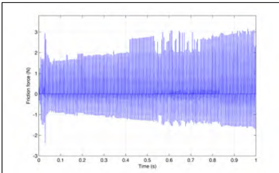
Figure-A II-11. Friction force at the crack interface
