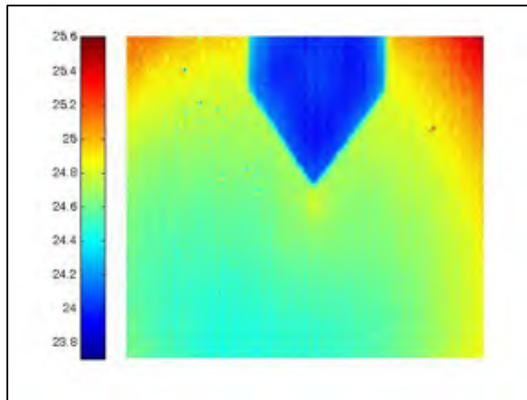
Figure-A I-5. Experimental temperature distribution at t=1s , 63 Hz excitation
