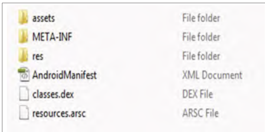
Figure 2.8 The component of apk package
