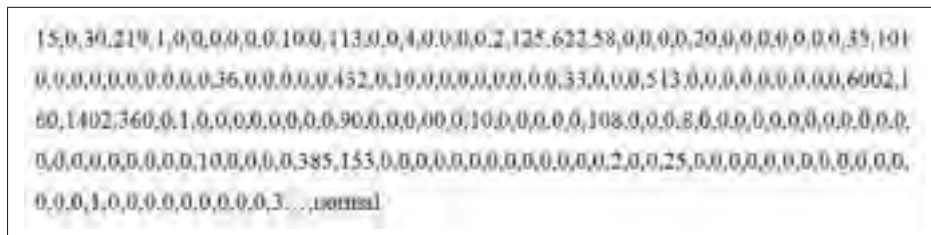
Figure 3.7 Pattern frequency system call feature vector
