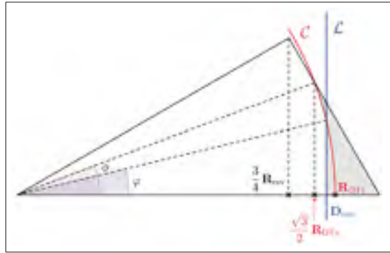
Figure-A II-1 Illustration of the Relay Efficiency Area for a half cell sector
