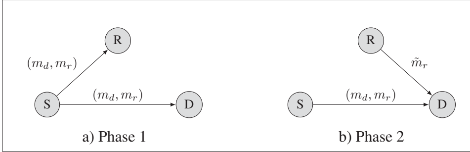
Figure 3.5 A general view of the proposed coding scheme
