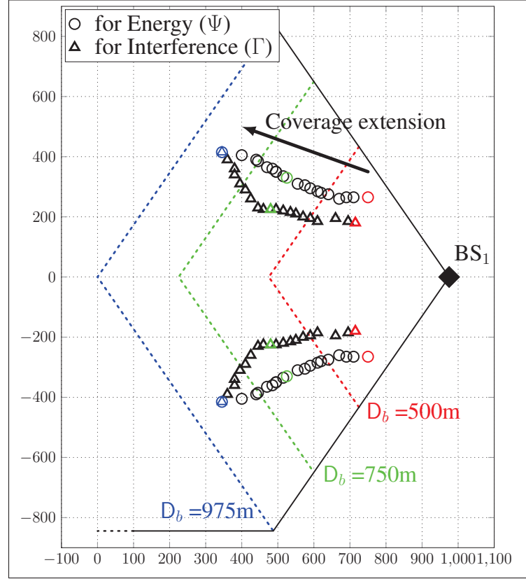
Figure 6.7 Optimal relay positions (N_r = 2, E_{2\text{Hop}}^{(\text{dsp})} = 50\text{mJ})
