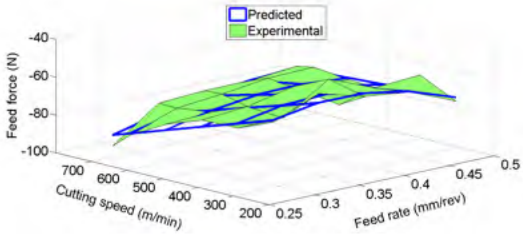
Fig. 11. Feed force for OP1 operation
