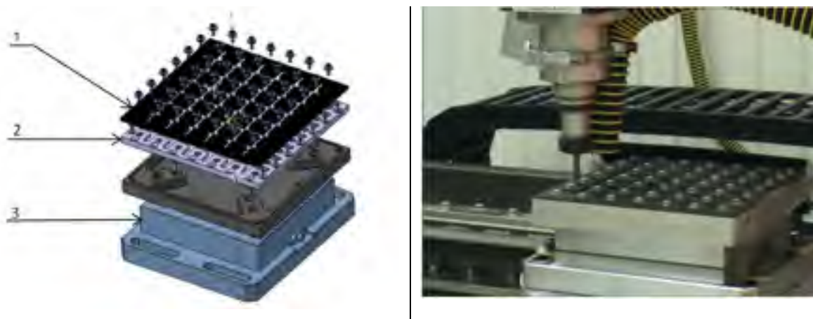
Fig. 5 Experimental set-up for dry trimming of CFRP
