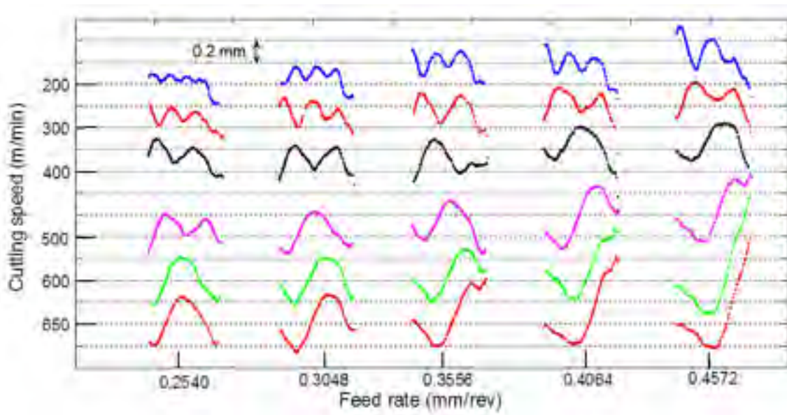
Fig.16 Comparison of trajectory deviations for OP1 operation
