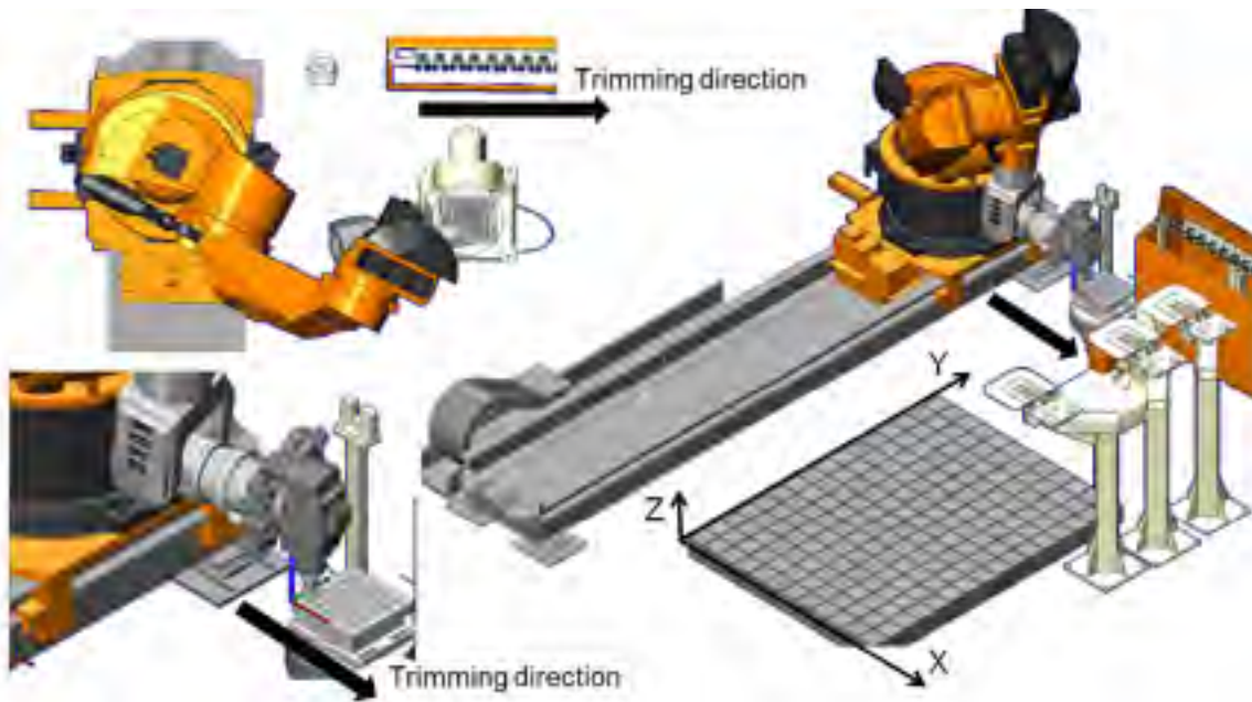
Fig. 3 Robot configuration during OP2 operation
