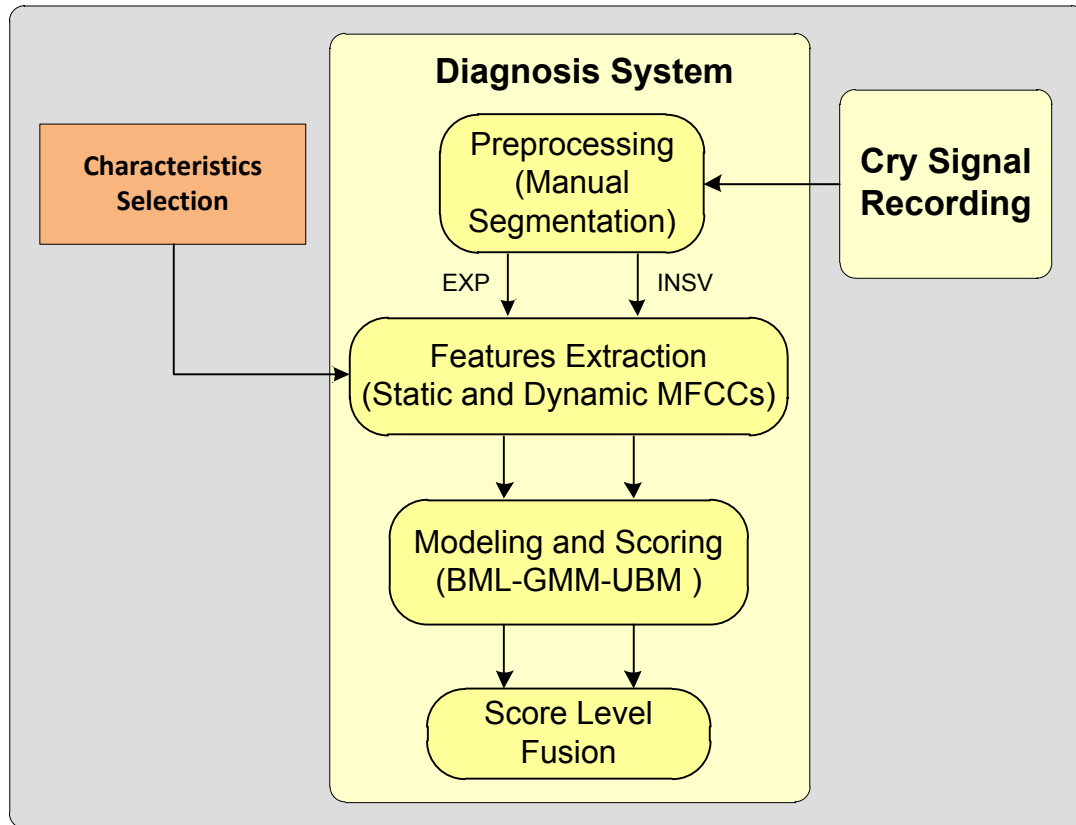
Figure 4.16 Introduced system overview
