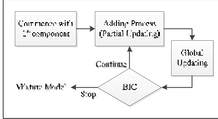
Figure 2.3 Block diagram of learning GMM using adapted BML technique
