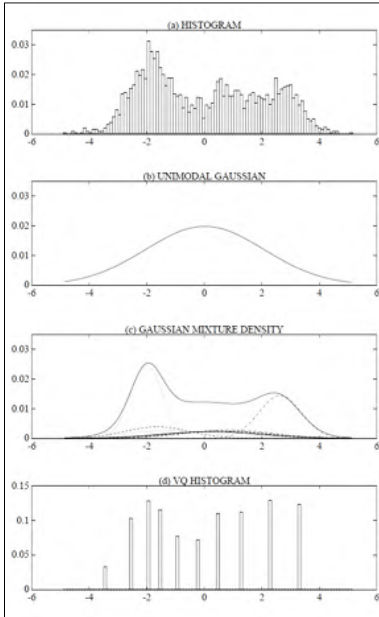
Figure 1.9 Obtained densities for uni-modal Gaussian model, GMM, and VQ
