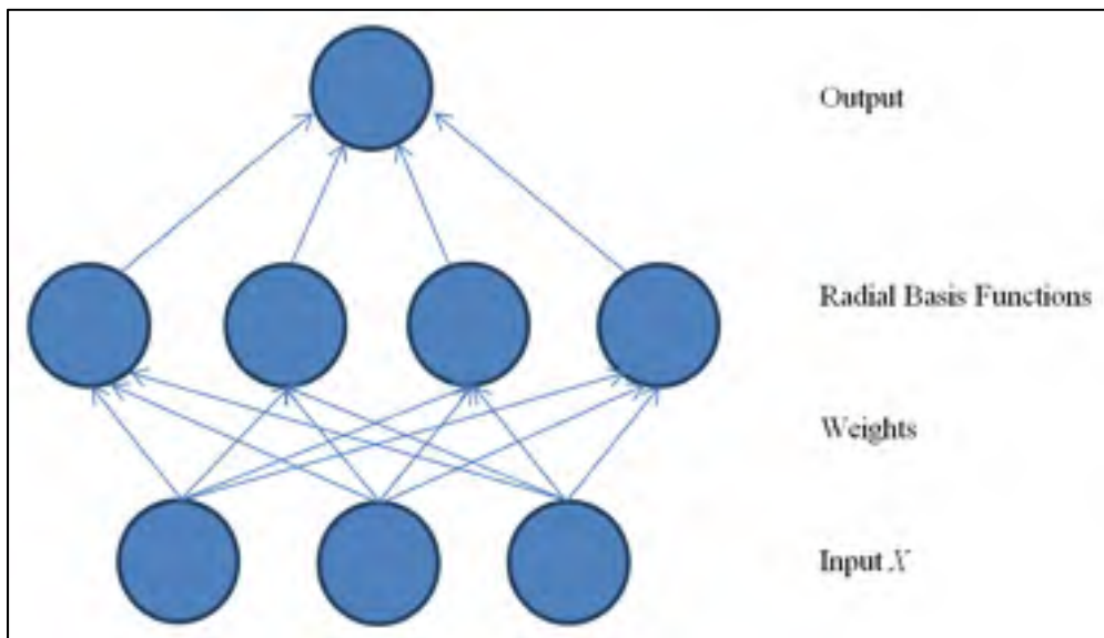
Figure 1.8 Structure of a basic RBF network
