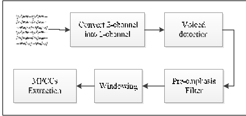
Figure 2.2 Pre-processing steps
