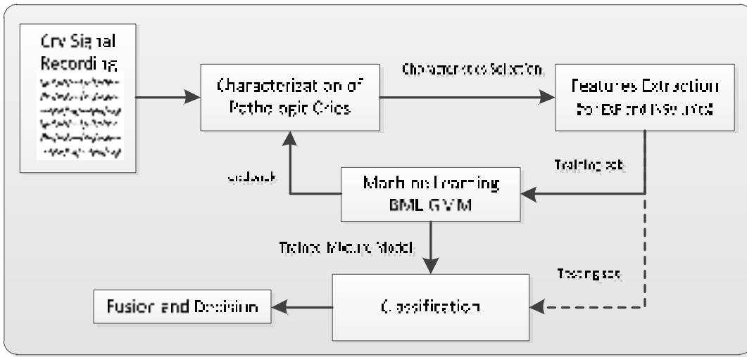
Figure 1.12 Modeling and decision
