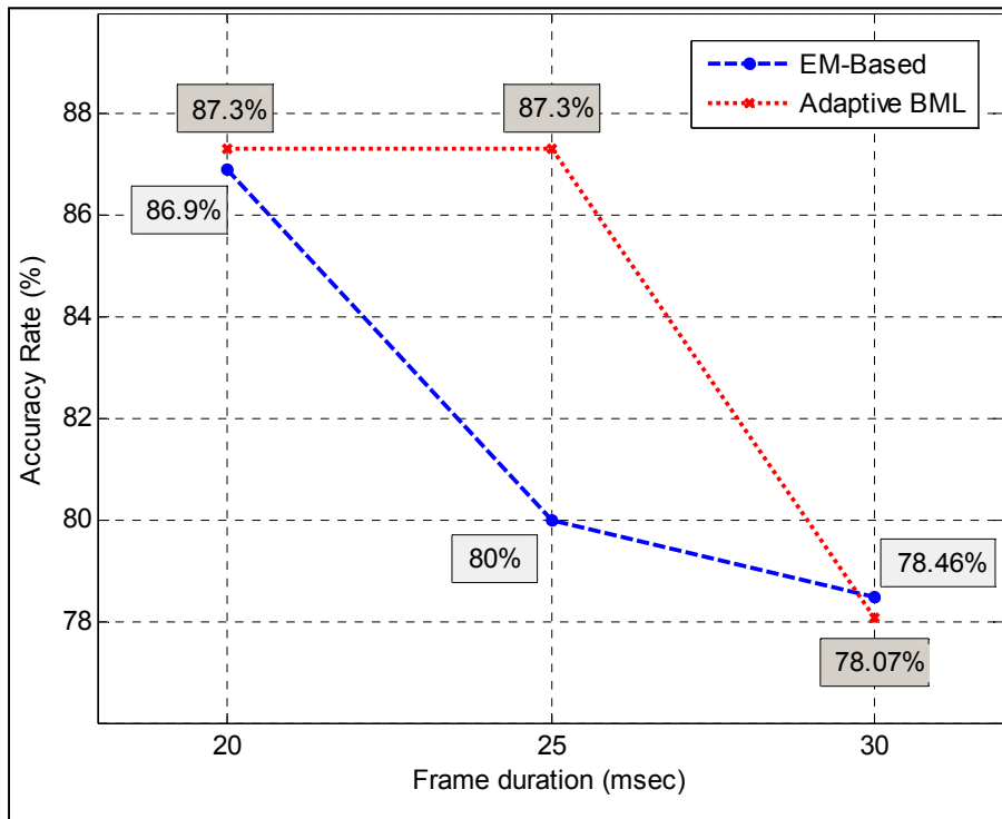
Figure 2.5 Mean classification accuracy rates
