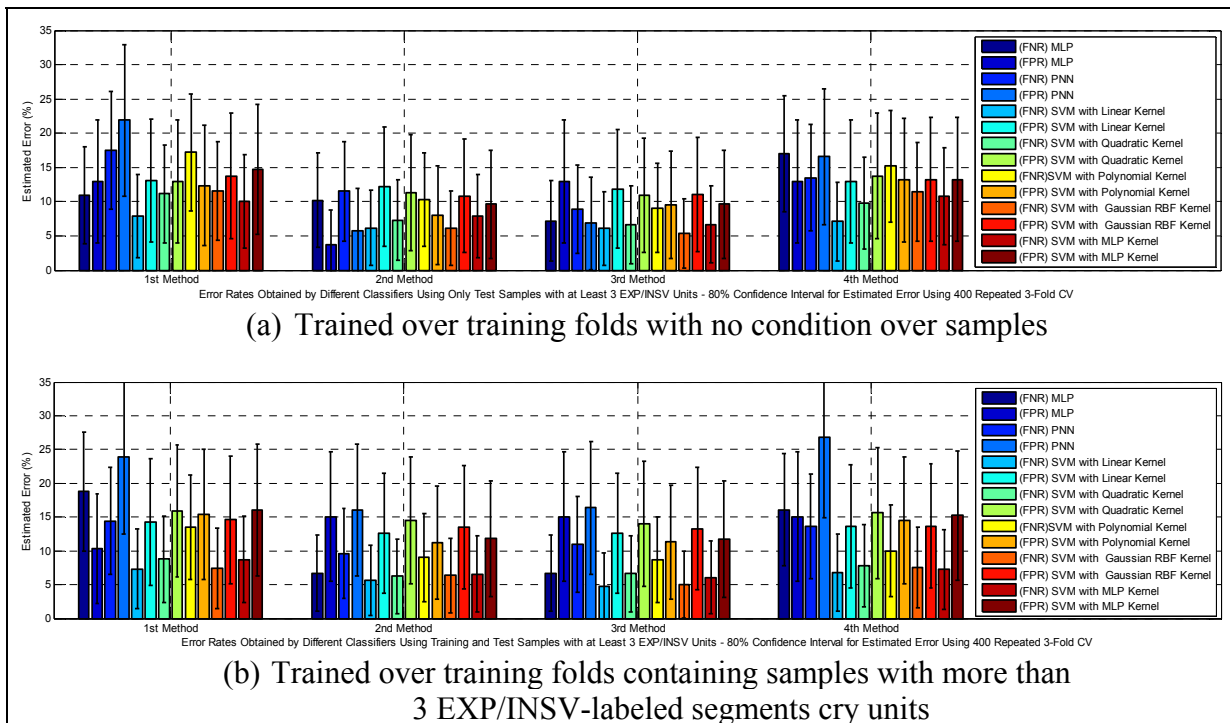
Figure 4.11 Type I and type II errors of the classifiers used in the healthy infant detection task using 400 repeated 3-fold CVs for the test samples that contain more than 3 EXP and INSV-labeled cry units
