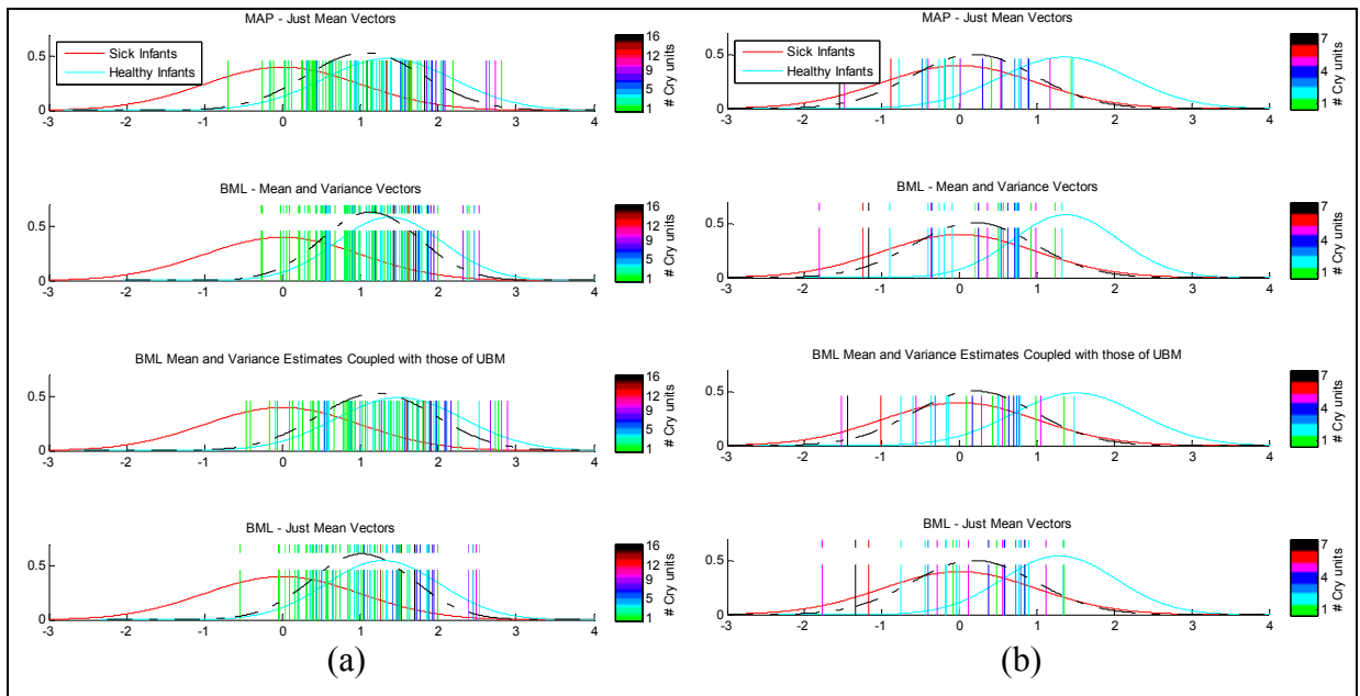
Figure 4.5 Mean of the LLR scores over INSV cry units inside the (a) healthy and (b) sick infants for the healthy infant verification system
