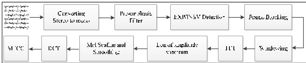
Figure 4.3 Pre-processing and MFCC feature extraction steps
