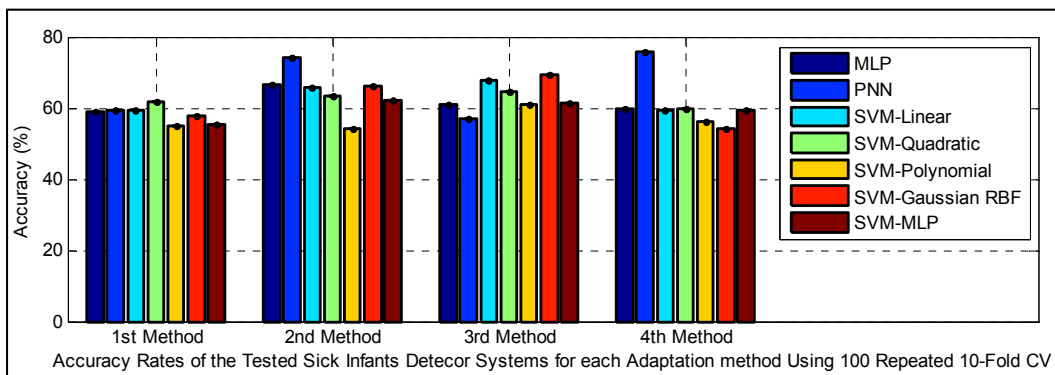
Figure 4.13 Comparison of the accuracy rates of all of the classifiers in the sick infant (affected by neurological problems) detection task
