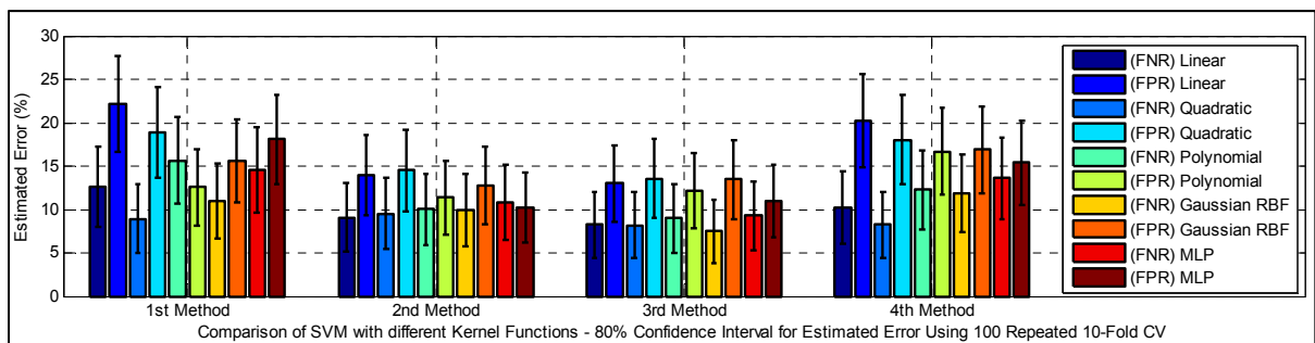
Figure 4.9 Type I and type II errors for the SVM with different kernel functions in the healthy infant detection task
