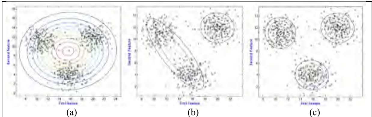
Figure 3.2 Estimated contour (a) of the first Gaussian component, (b) after splitting GMM into 2 components, (c) of final GMM
