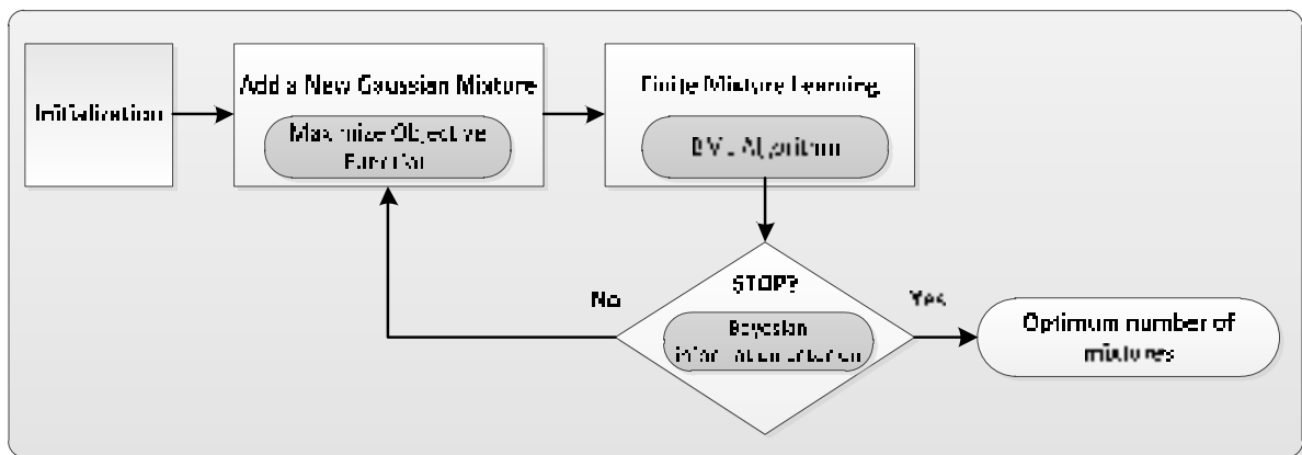
Figure 1.11 The growing process of finite mixture model
