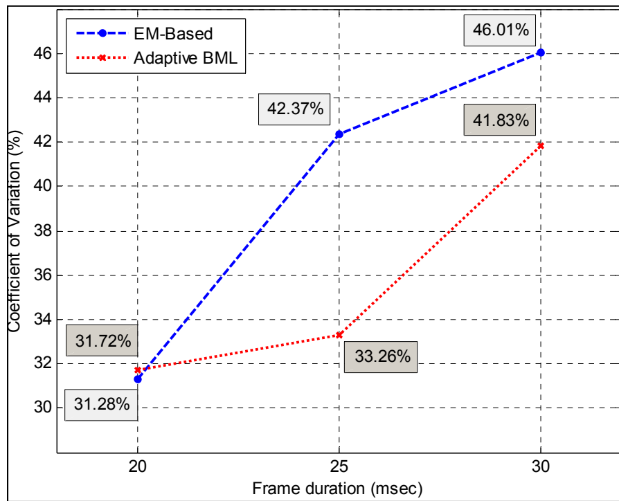
Figure 2.6 Coefficient of variation
