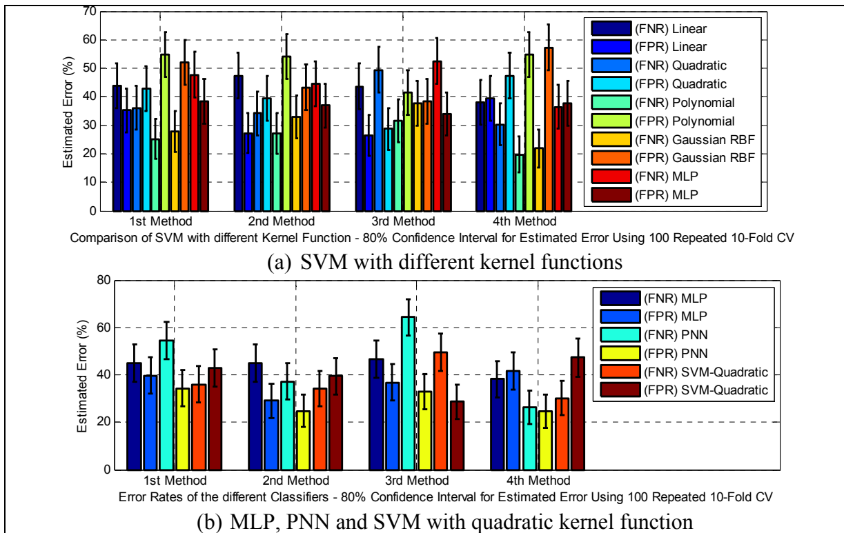
Figure 4.12 Type I and type II errors for the different classifiers in the sick infant (affected by neurological problems) detection task
