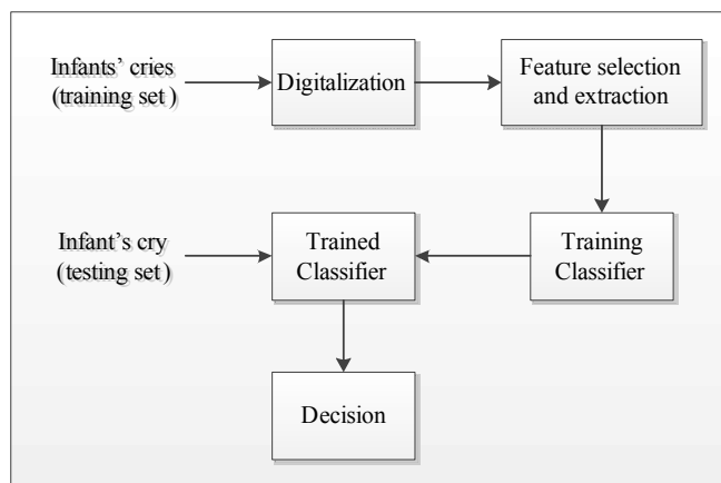
Figure 1.6 Block diagram of auto diagnostic system by using pattern recognition
