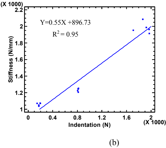
Figure 4. Relationships between Indentation and: (a) pullout; (b) stiffness
