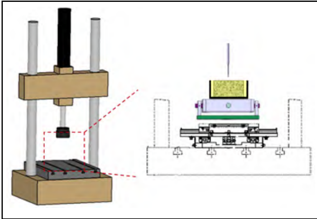
Figure 3.5 Experimental apparatus used for pilot hole creation into synthetic bone specimen
