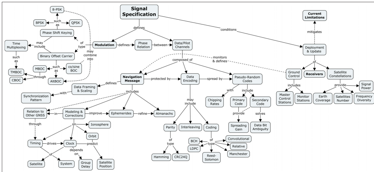
Figure 2.1 GNSS Signals
