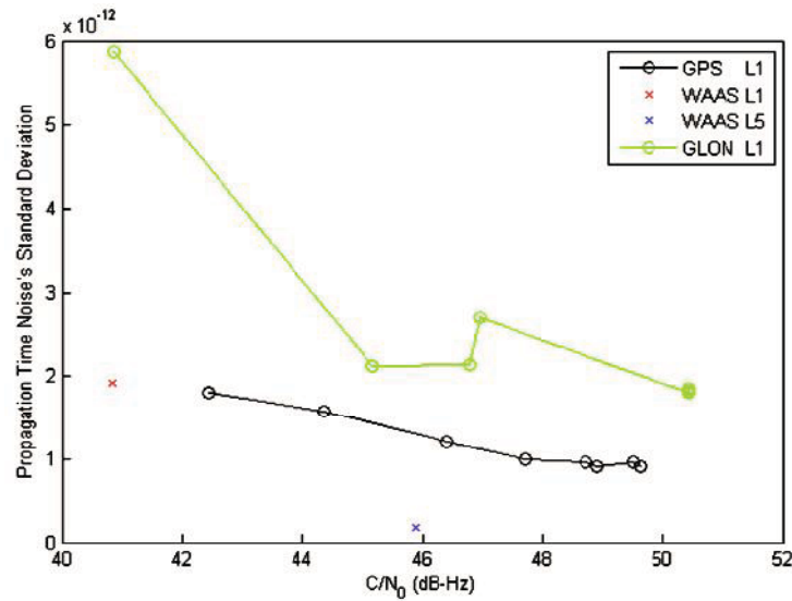
Figure 3. Correlator spacing impact on DLL noise vs. C/N_0 .
