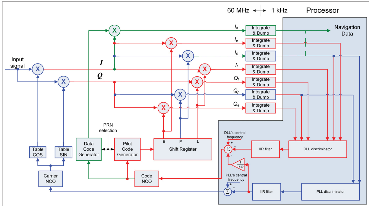
Figure 1.8 BPSK Tracking Loop PLL [blue], DLL [red], Data [green]
