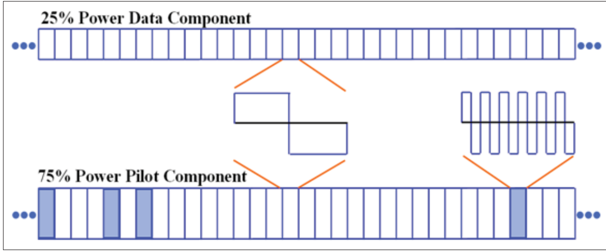
Figure 2.7 TBOC Pilot Sub-Carriers Assignment Pattern Adapted from ARINC Engineering Services (2013, Figure 3.3-2)
