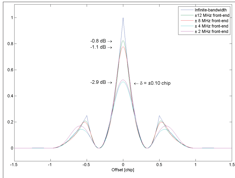
Figure 1.10 Non-Coherent (Power) Bandwidth-Limited Normalized BOC(1, 1) ACF of a Square Chip
