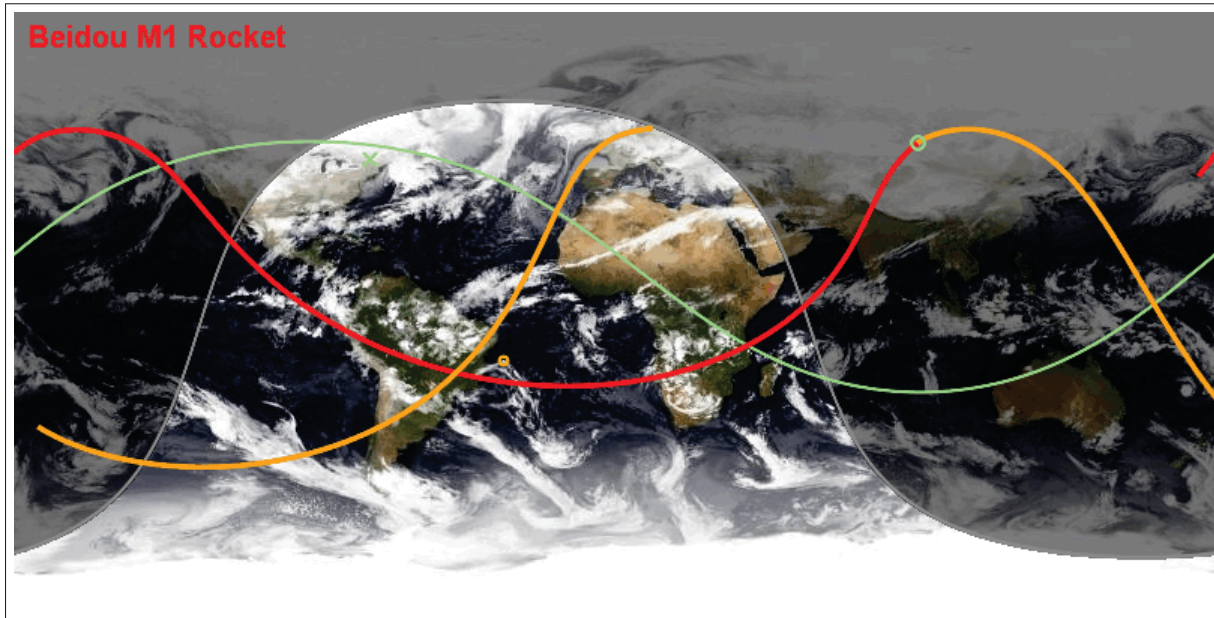
Figure 2.12 Ground Track of COMPASS-M1 MEO Satellite over 24 h Taken from Barmettler (2015)
