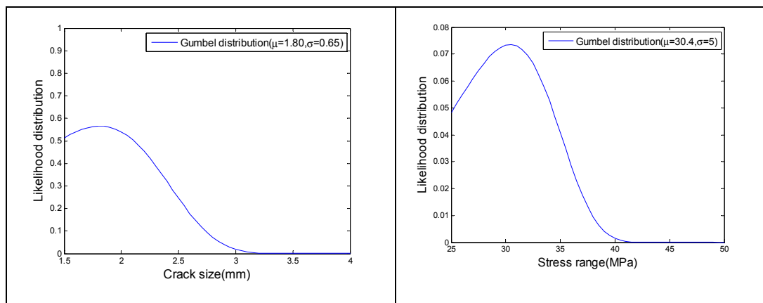
Figure 2.4: Likelihood distribution
