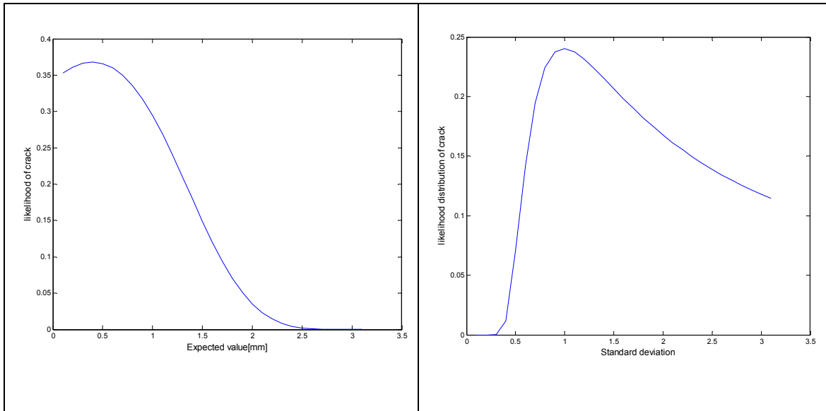
Figure 2.12: Likelihood distribution for crack size
