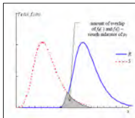
Figure 3.1: Basic failure problem (VĂCĂREANU, ALDEA et al. 2007)
