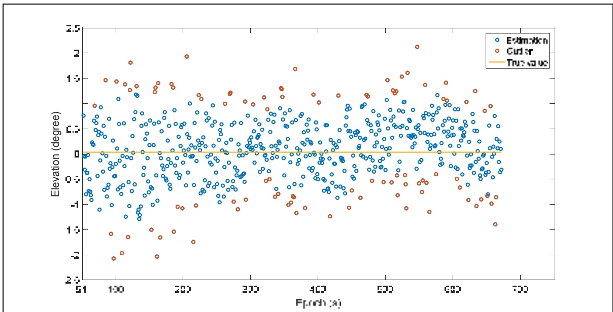
Figure 5.18 Elevation estimation and the detected outliers in test case 2
