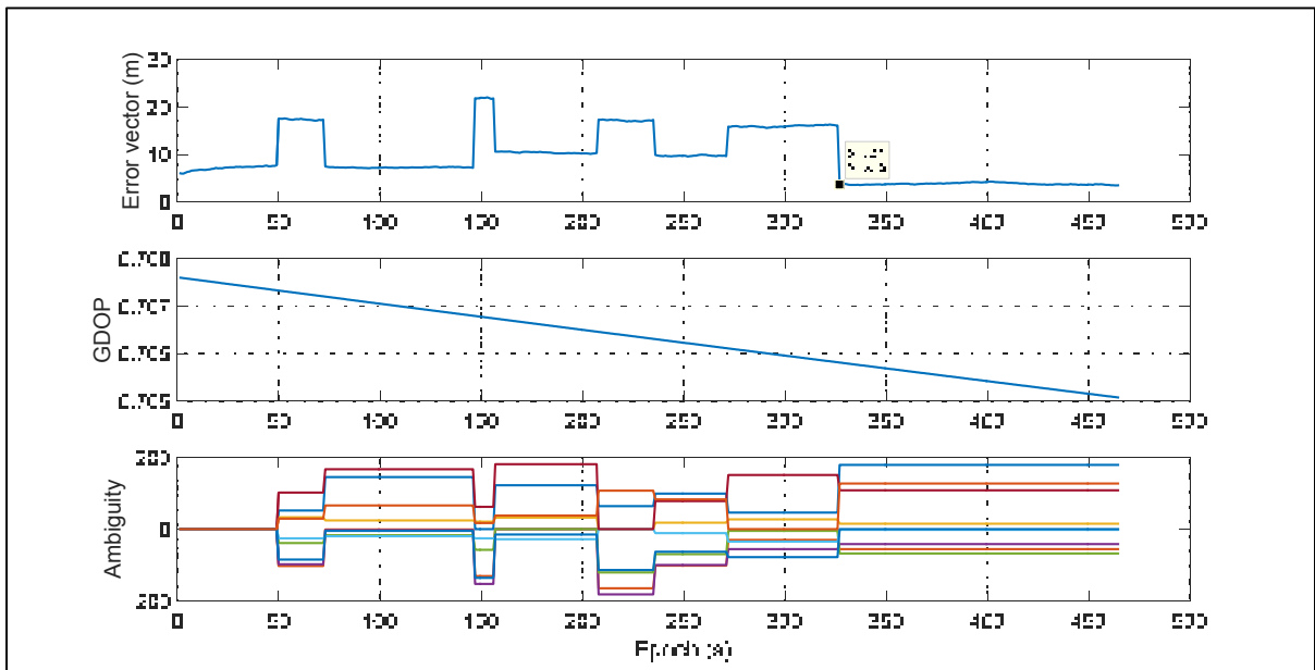
Figure 5.23 Relation between the estimation error, GDOP and the ambiguities in test case 3
