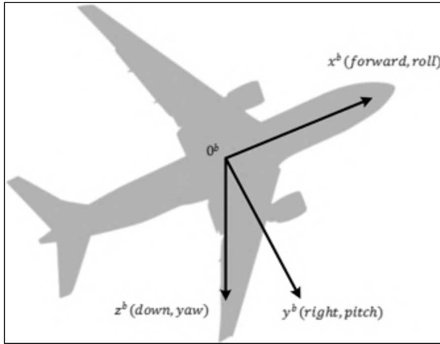
Figure 2.12 Body frame
