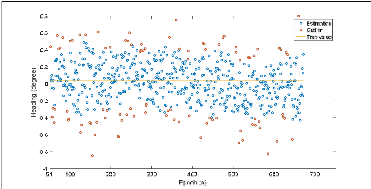
Figure 5.17 Heading estimation and the detected outliers in test case 2
