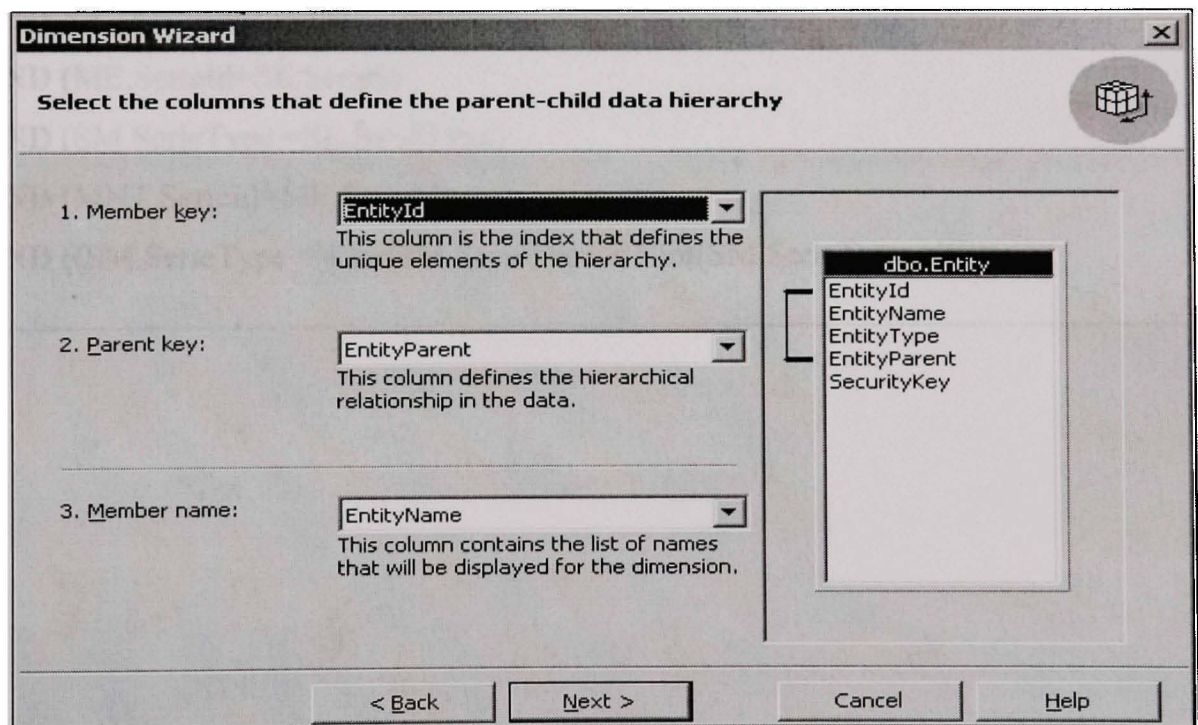
Figure X.6 Parent-child data hierarchy.
