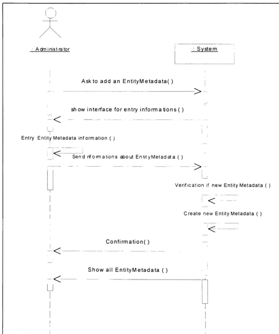
Figure X.3 Sequence diagram - Add an EntityMetadata.
