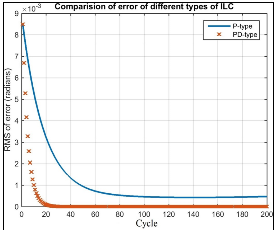
Figure 5.14 Comparison of two types of ILC according to the RMS error convergence
