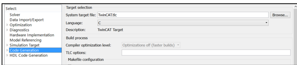
Figure 6.4 Configuring Simulink for TwinCAT file generation
