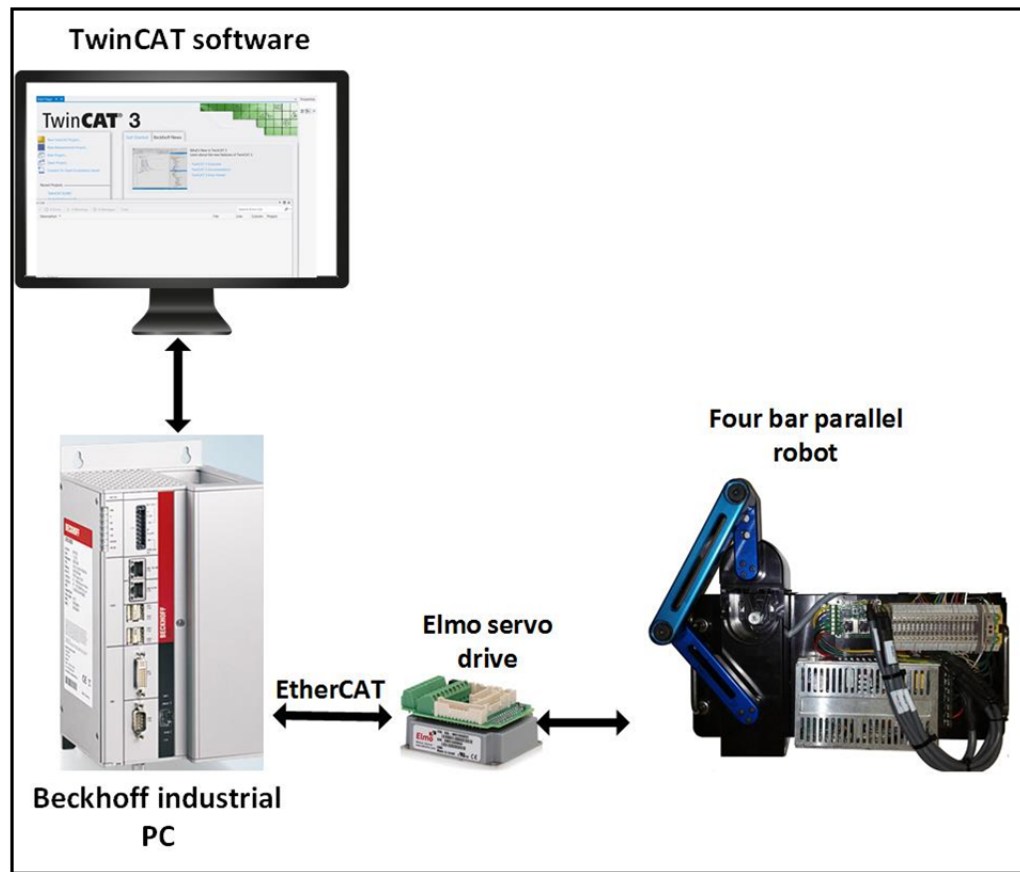
Figure 6.5 Robot setup
