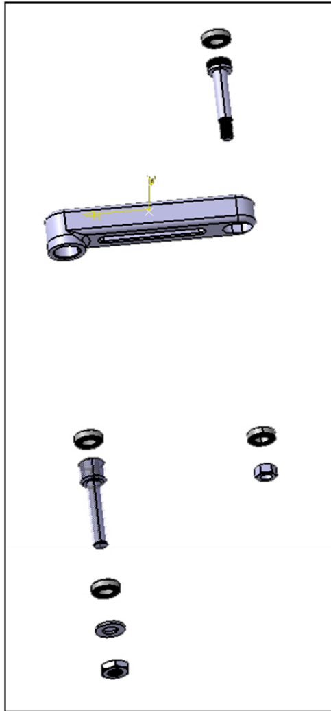
Figure 3.2 Exploded view of parts for the third link subassembly
