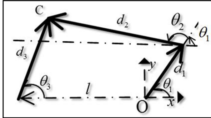
Figure 2.3 Vector representation of robot in Cartesian space
