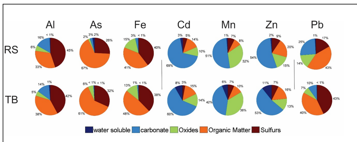
Figure 2.6 SDM results, grouped by trace metal separated between Rio Santa and tributaries. Trace metals have been grouped into three clusters, depending on the dominant phases in the Rio Santa and tributaries sediments. Al, As, Fe form the first cluster; Cd, Mn, Zn, the second cluster, and Pb, the third cluster
