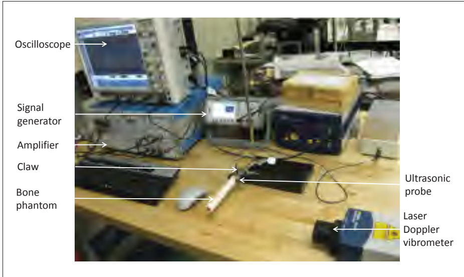
Figure 3.3 Experimental setup.
