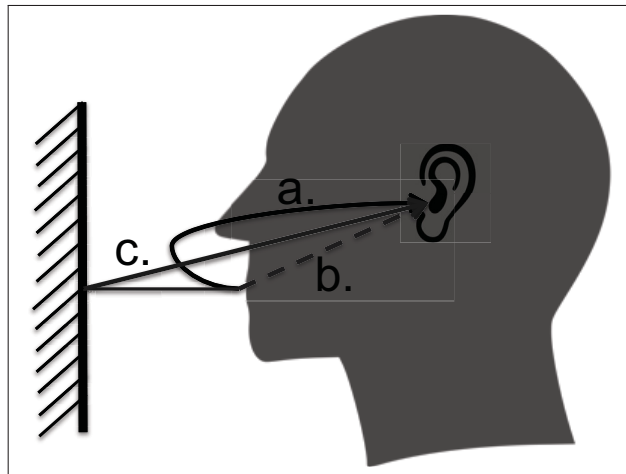
Figure 1.2 Illustration of the three paths affecting the perception of one's own voice: (a) direct air-conduction, (b) bone-conduction, and (c) indirect air-conduction.
