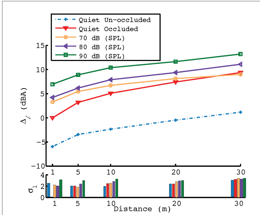
Figure 3.5 Average increase in speech levels, \Delta_I from the occluded quiet condition over increasing distance and noise levels. The level at 1 m distance for the quiet occluded condition is used as reference for all the curves. The standard deviation, \sigma_I , in \Delta_I across talkers over different noise conditions and distance.
