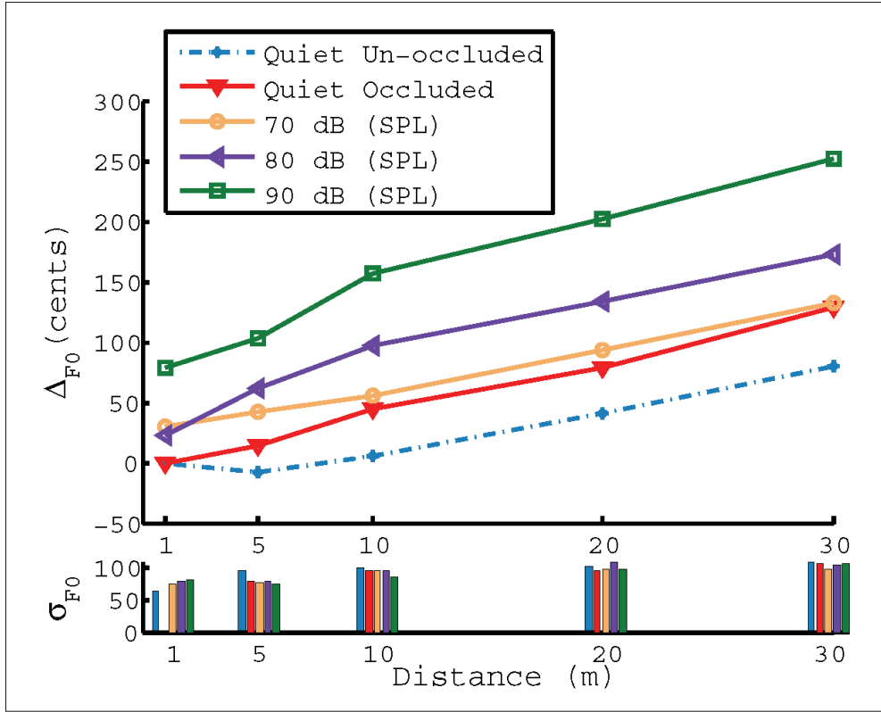
Figure 3.6 Average increase in F0 level, \Delta_{F0} , from the occluded quiet condition over increasing distance and noise levels. F0 at 1 m distance for the quiet occluded condition is used as reference for all the curves. The standard deviation, \sigma_{F0} , in \Delta_{F0} across talkers over different noise conditions and increasing distance.
