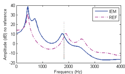
FIGURE 2: IEM vs. REF spectral envelopes of the utterance /u/ from the word 'canoe', showing the increased low frequency content and the missing high frequency content.
