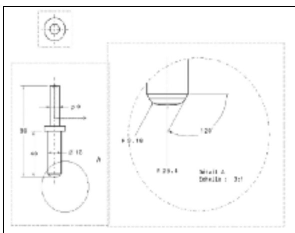
Figure 3.5 Outil de martelage (dimensions en mm) (Laroche et al., 2002)
