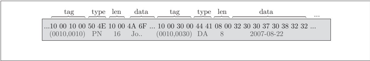
Figure 1.9 DICOM binary format
