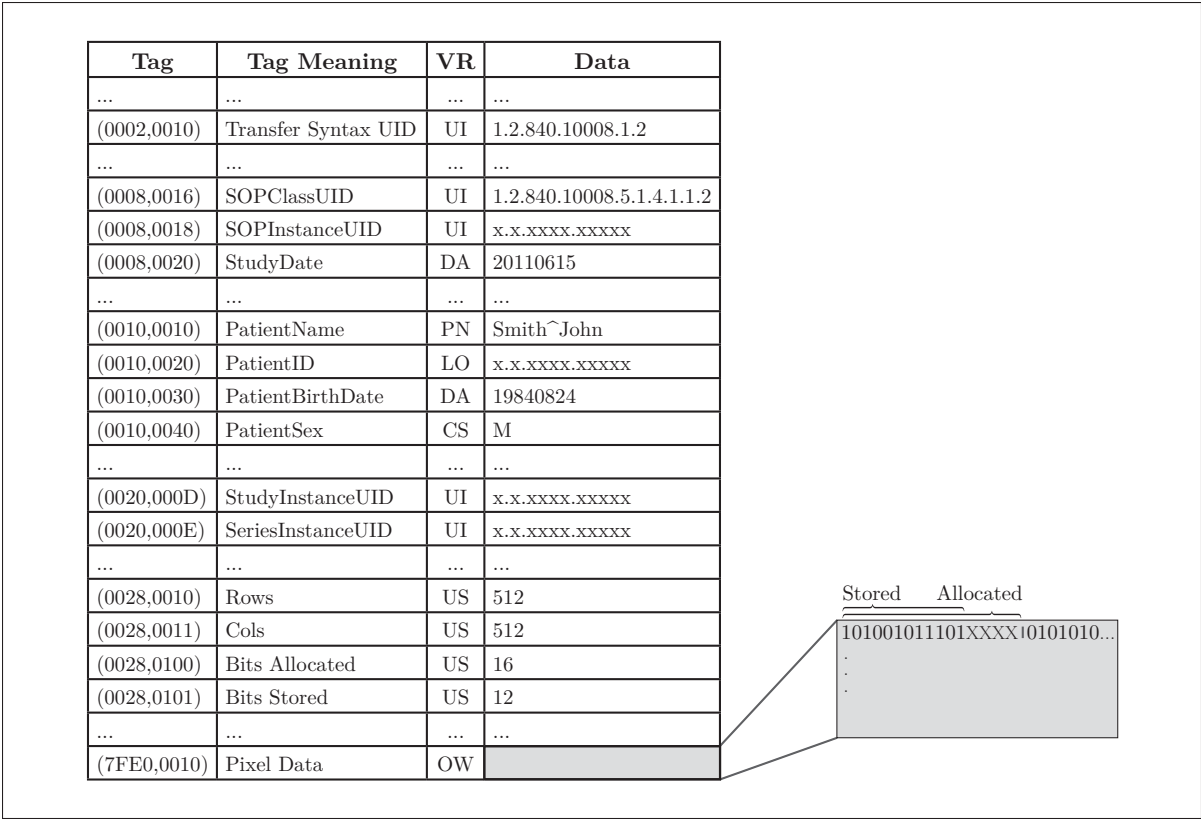
Figure 1.8 DICOM with RAW pixel data
