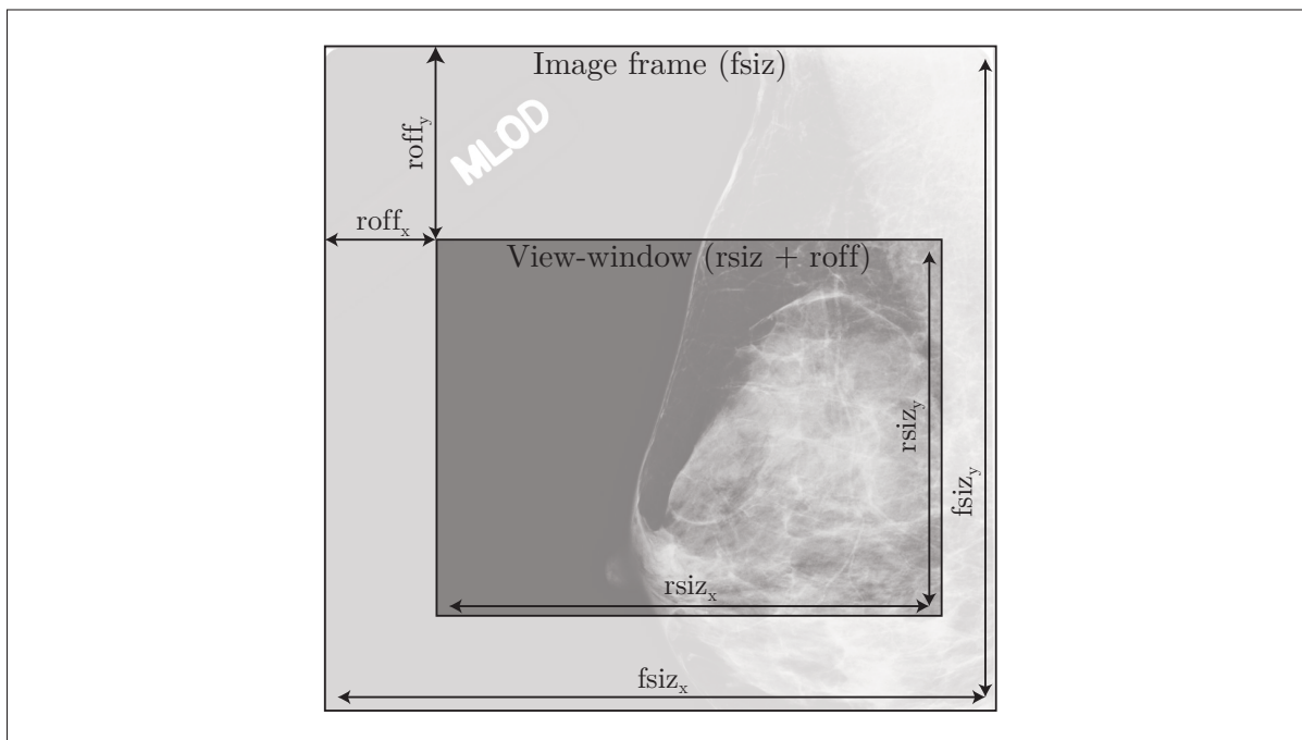
Figure 1.7 JPIP View-Window
