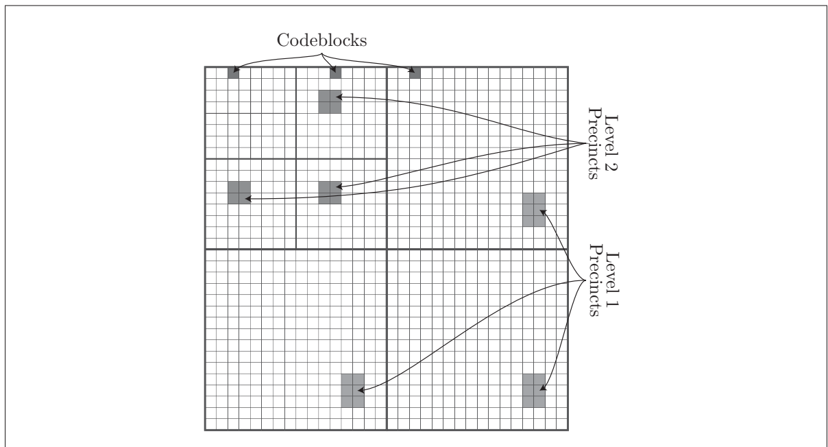
Figure 1.5 Codeblocks and precinct organization
