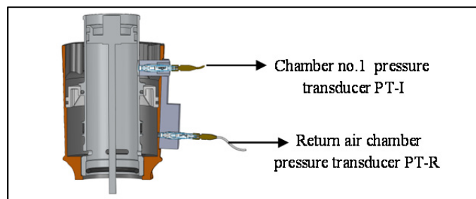
Figure 4.11 Section view of the nailer instrumented with pressure transducers
