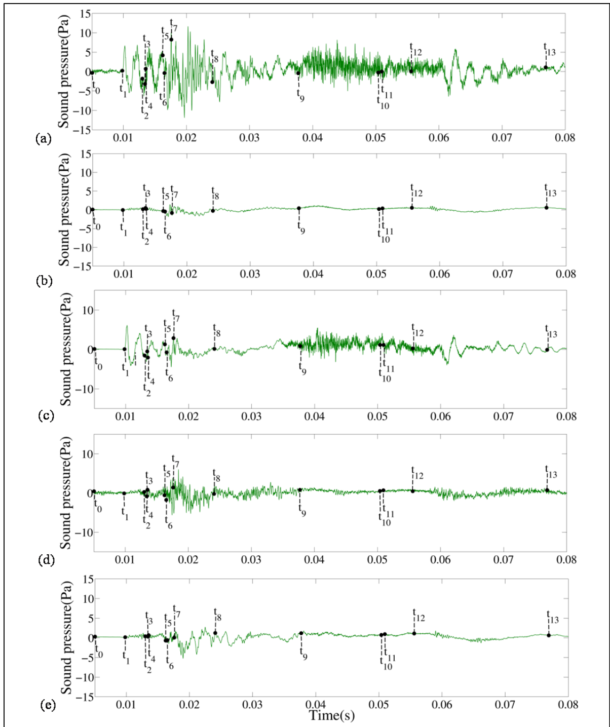
Figure 1.11 Sound pressure Microphone no. 5: (a) Total noise (Conf.W-1), (b) Residual noise (Conf.W-2), (c) Air exhaust noise (Conf.W-3), (d) Machine body noise (Conf.W-4), (e) Workpiece/worktable noise (Conf.W-5)
