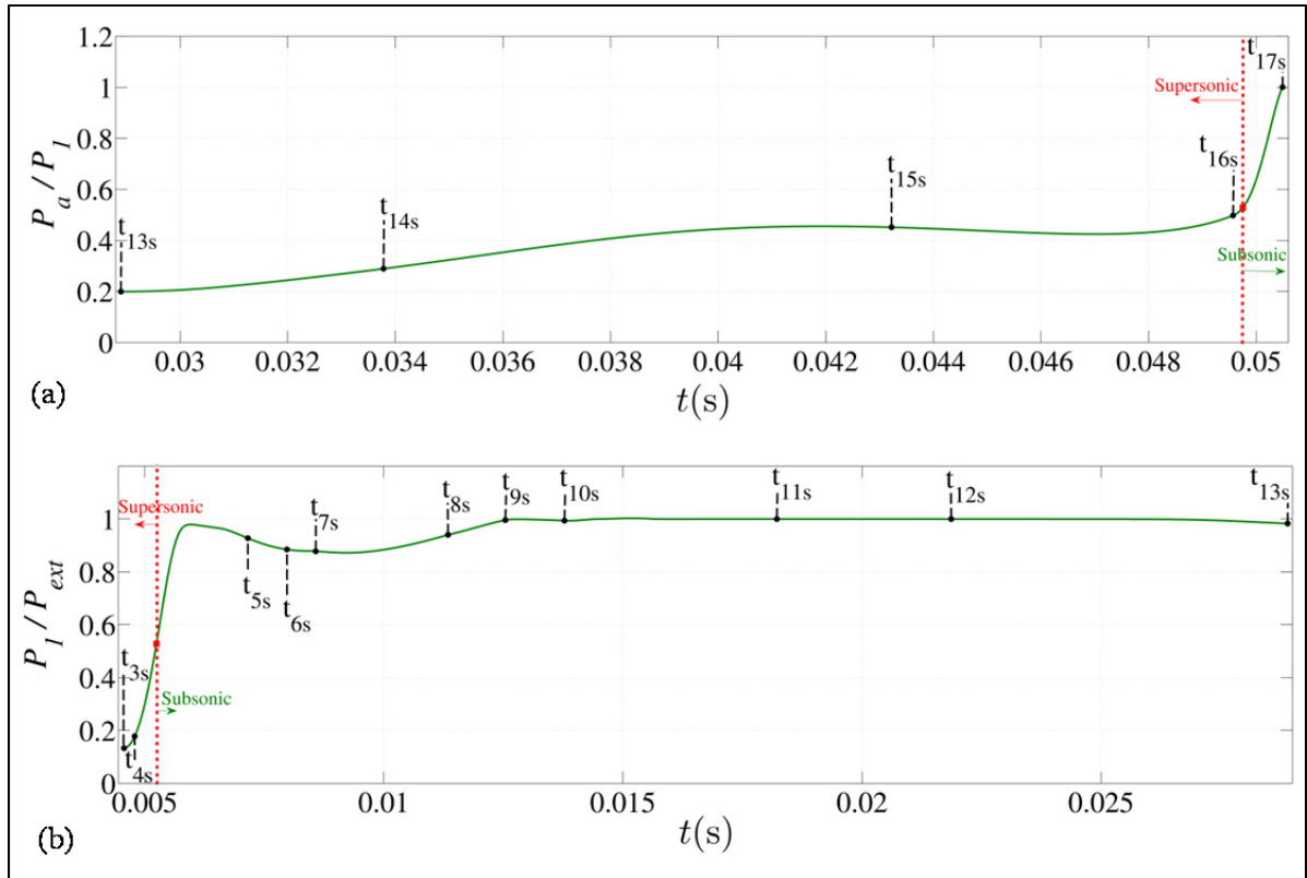
Figure 4.15 Downstream-to-upstream pressure ratio: (a) P_a/P_l , (b) P_l/P_{ext}
