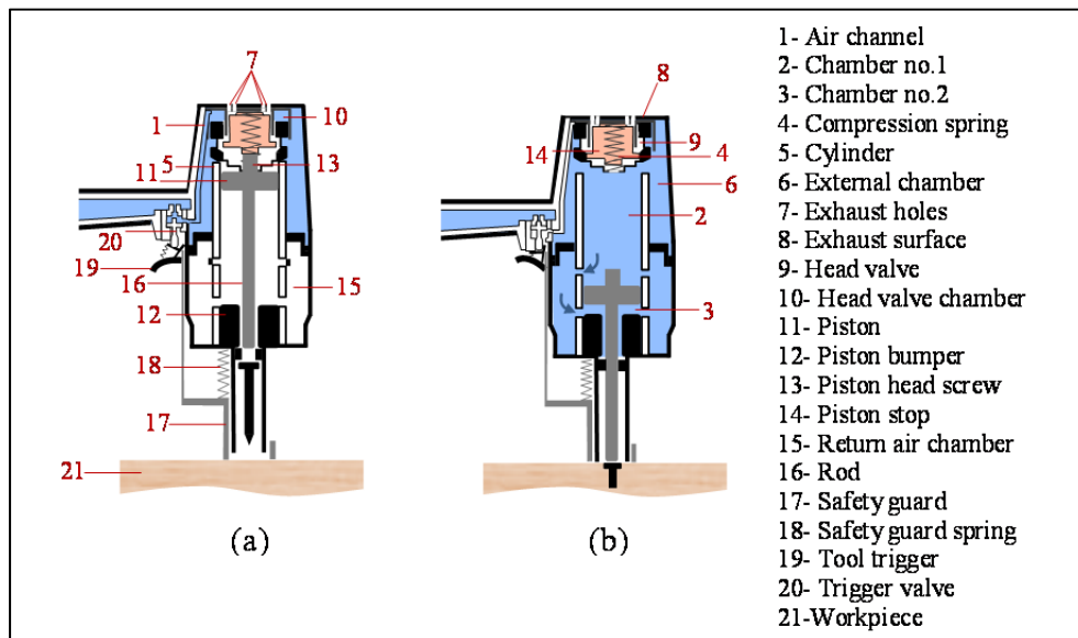
Figure 1.1 Schematic representation of a pneumatic nailing device: (a) at rest, (b) during the driving stroke
