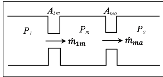
Figure 4.5 Exhaust restrictions
