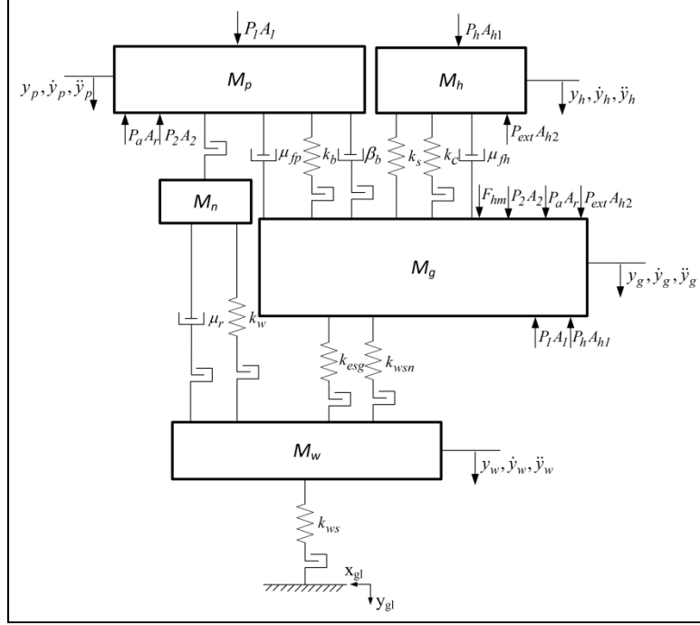
Figure 4.3 Pneumatic nailing device dynamic model.
