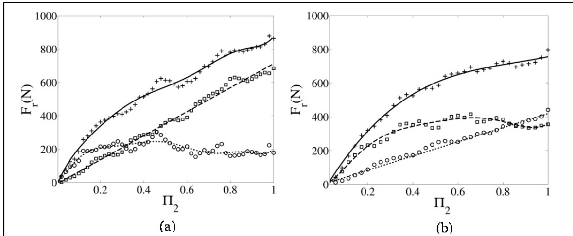
Figure 2.5 F_r constituents (wood type: PP, v=8.33 \times 10^{-3} m/s): (a) Smooth nails ( \Pi_4=0.0600 ), (b) Annularly threaded nails ( \Pi_4=0.0733 ). Solid line and cross: F_r fitted model and data; Dashed line and square: Friction force fitted model and data; Dotted line and empty circle: Deformation-fracture force fitted model and data
