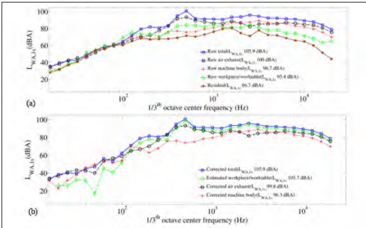
Figure 1.12 1/3 octave band analysis for worktable setup: (a) raw data, (b) corrected data
