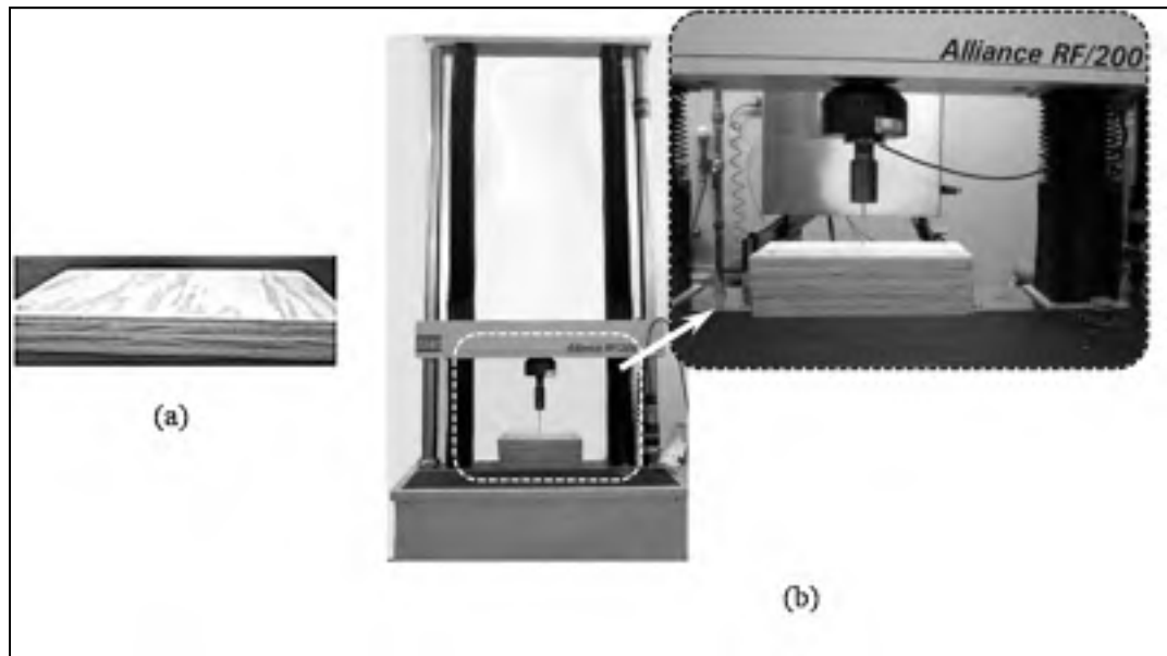
Figure 2.1 (a) Douglas-Fir plywood panel, and (b) experimental set-up
