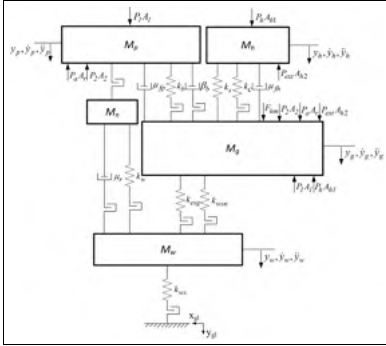
Figure 4.3 Pneumatic nailing device dynamic model. Nonlinear elements: \mu_r, k_w, \mu_{fp}, k_b, \beta_b, k_c, \mu_{fn}, k_{esg}, k_{wsn}, k_{ws}, and k_s .
