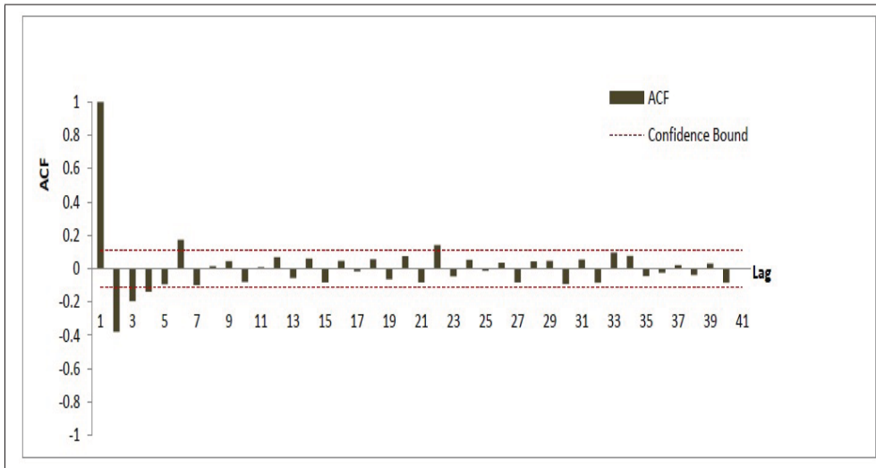
Figure 4.4 ACF Function of the Differenced Data at d = 1
