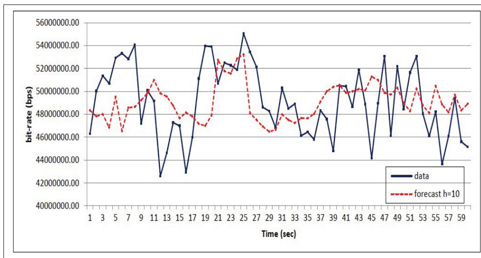
Figure 6.9 Forecast results with h = 10
