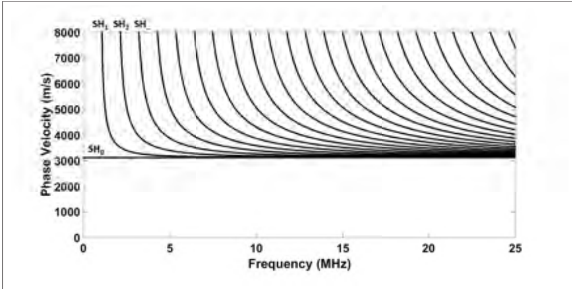
Figure 1.3 Phase velocity dispersion curves of the SH waves in a 1.588 mm aluminum plate ( E = 70.8 GPa, \nu = 0.34 , and \rho = 2700 kg/m 3 ), curves computed using DISPERSE software packages (Pavlakovic et al. (1997))
