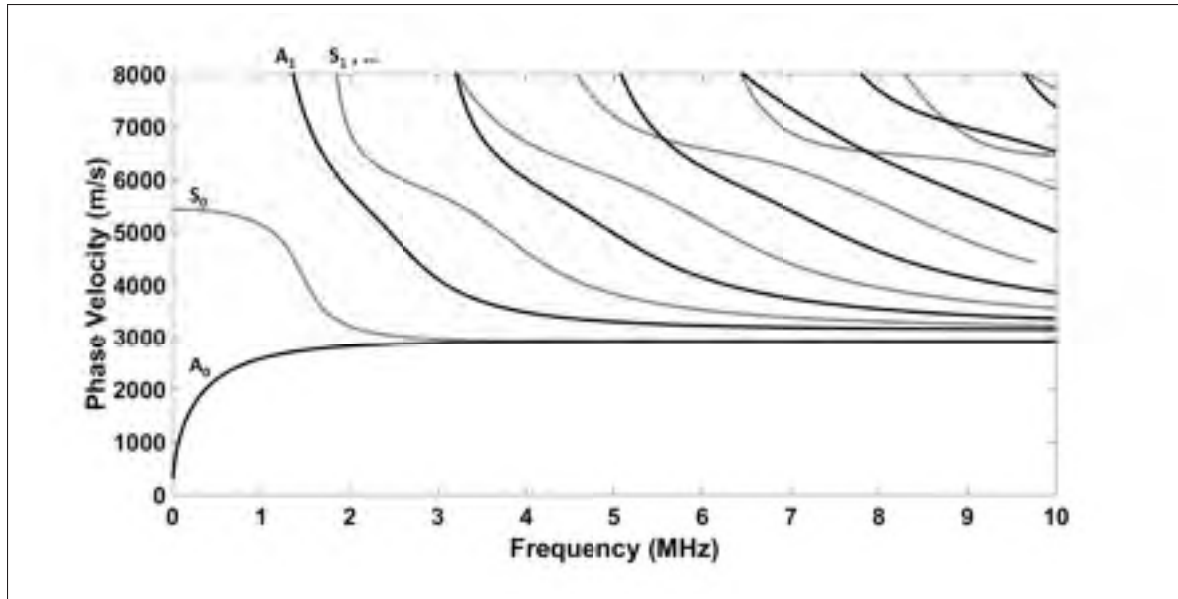
Figure 1.6 Phase velocity dispersion curves of Lamb waves in a 1.588 mm aluminum plate ( E = 70.8 GPa, \nu = 0.34 , and \rho = 2700 kg/m 3 ), curves computed using DISPERSE software packages (Pavlakovic et al. (1997))
