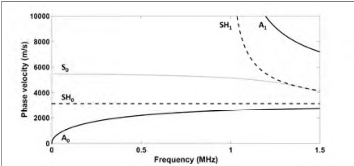
Figure 2.1 Phase velocity dispersion curves in a 1.59 mm aluminum plate ( E = 70.8 \text{ GPa} , \nu = 0.34 , and \rho = 2700 \text{ kg/m}^3 ). The solid black lines correspond to the A_0 and A_1 modes, the solid light-grey lines correspond to the S_0 mode and the dashed black lines correspond to the SH_0 and SH_1 modes
