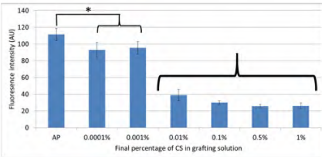
Figure 4.28 Protein adsorption on amine plate based bioactive coatings prepared using different percentages of CS in the grafting solution. Results are presented as fluorescence intensity units (N=1, n=4, representative of 2 independent experiments) (* p < 0.05 )
