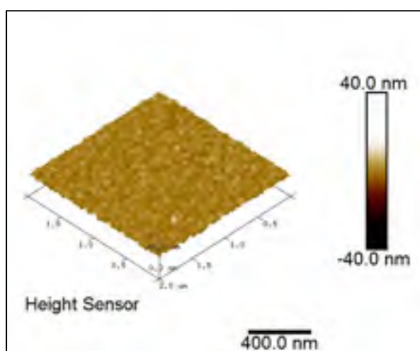
Figure 4.11 AFM height measurements 3D image for LP+CS sample (2 μm x 2 μm)
