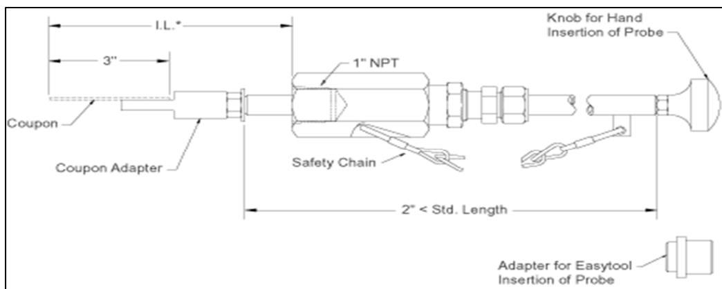
Figure 2.4 Porte-coupon de corrosion RT4000 (Metal Samples Company, 2014)
