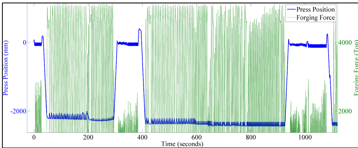
Figure 28 : Finishing characterisation
