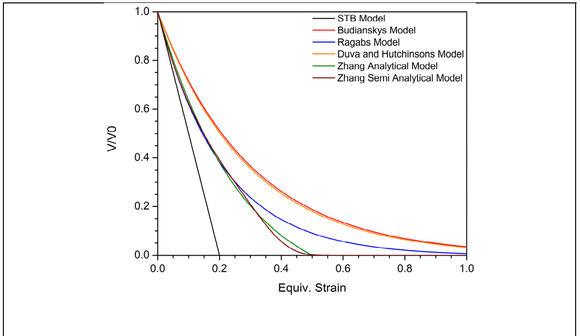
Figure 39 : Void closure comparison for 14NiCrMo13, T_x = -1 .
