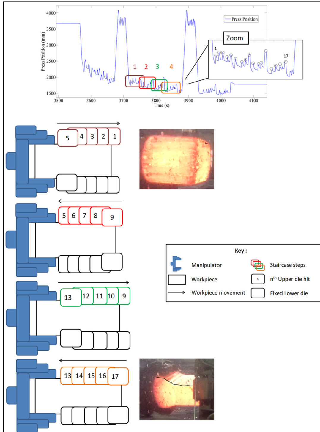
Figure 27 : Example of Staircase Forging
