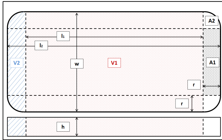
Figure 60 : Billet final volume schematic
