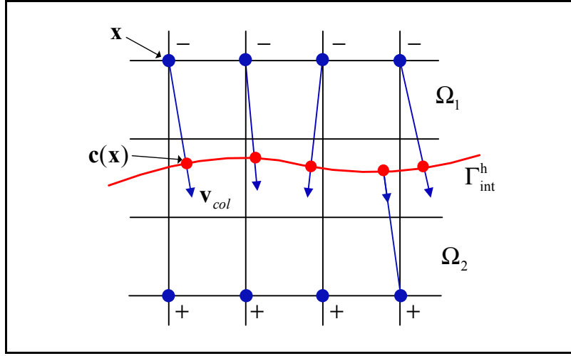
Figure 4.3 Closest point. Blue dots are grid points with their corresponding closest point \mathbf{c}(\mathbf{x}) on the interface as red dots. Collinear vectors \mathbf{v}_{col}(\mathbf{x}) are drawn from \overline{\mathbf{x}\mathbf{c}(\mathbf{x})} . ”+” and ”-” indicate the signs of the level set nodal values
