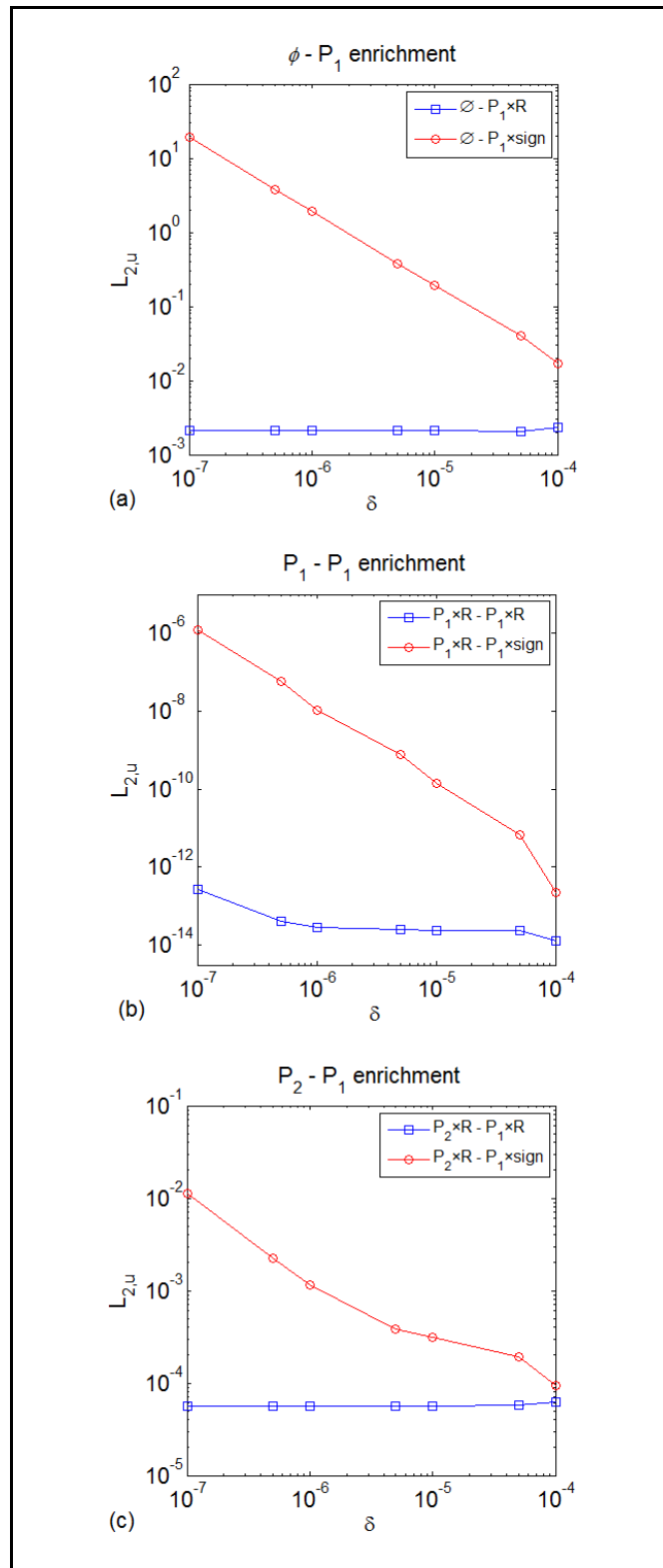
Figure 6.7 Two-phase Poiseuille: influence of an ill-conditioned system
