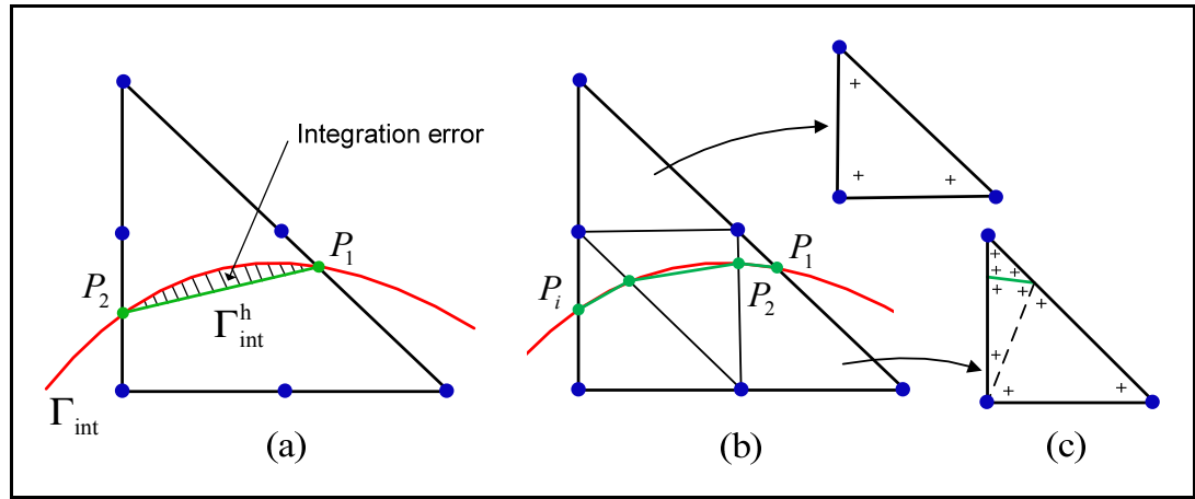
Figure 3.3 Curved interface inside a quadratic element and integration error committed with the linear approximation of the interface. In green, the approximated interface and computed points P_i on the interface
