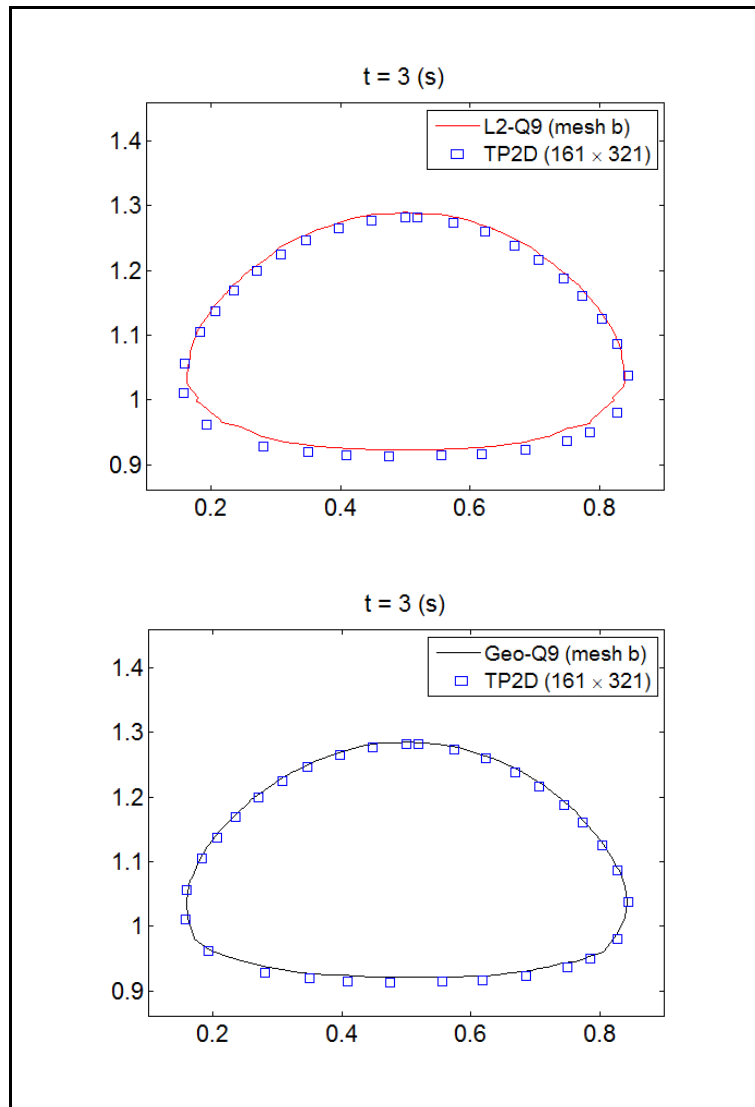
Figure 6.33 Rising bubble: final shape of the bubble at t = 3 \text{ s} and reference solution by Hysing et al. (Hysing, Turek et al. 2009)
