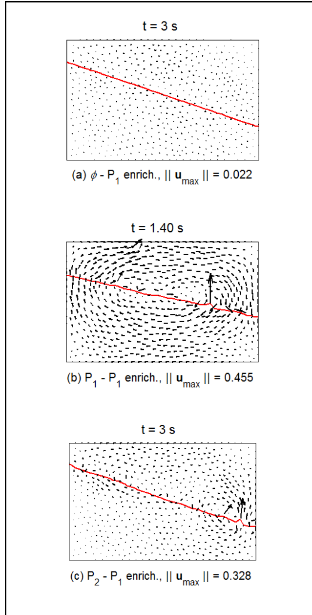
Figure 6.16 Parasite velocities: the \phi - P_1 enrichment (a) performs better than the P_1 - P_1 (b) and the P_2 - P_1 (c) enrichments
